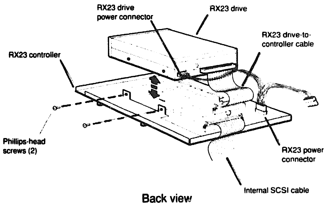
Figure 21. Removing and installing an RX23 drive controller
