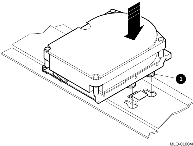
Figure 2–11 Inserting an RF3x-EK Hard Disk Drive in the Expander Box
