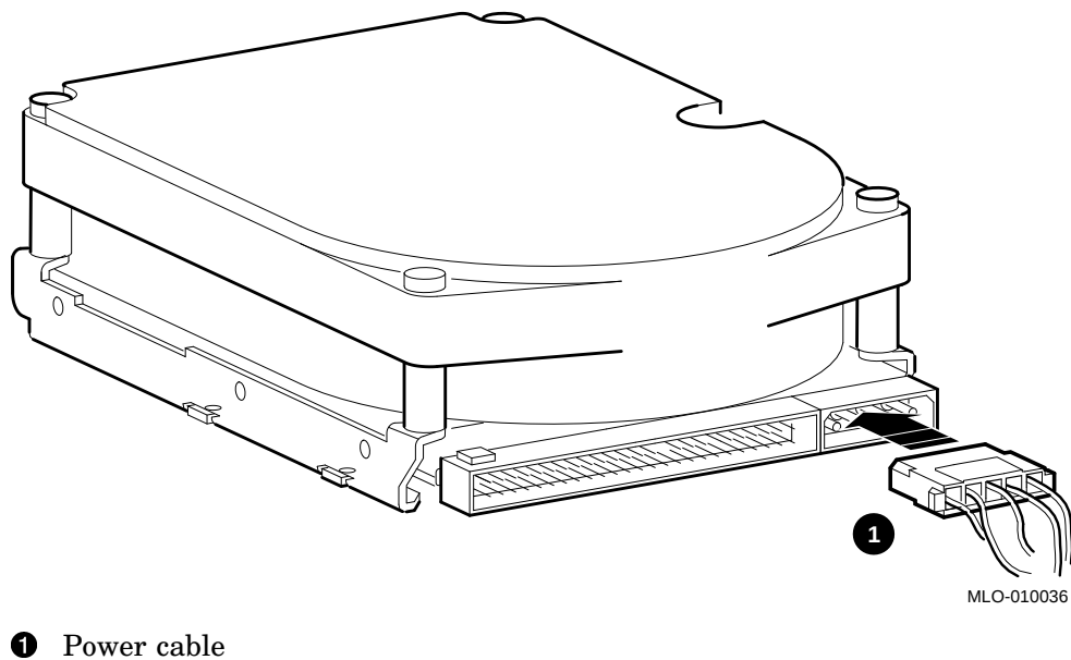
Figure 2–6 Connecting the 5-Pin Power Cable
