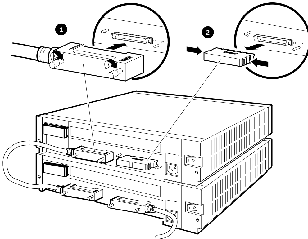
Figure 1–12 Connecting the Three-Foot DSSI Cable and Terminator to the Final Expender
