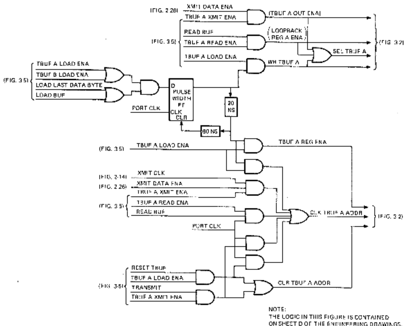
Figure 3-7 TBUF Sequencing Logic
