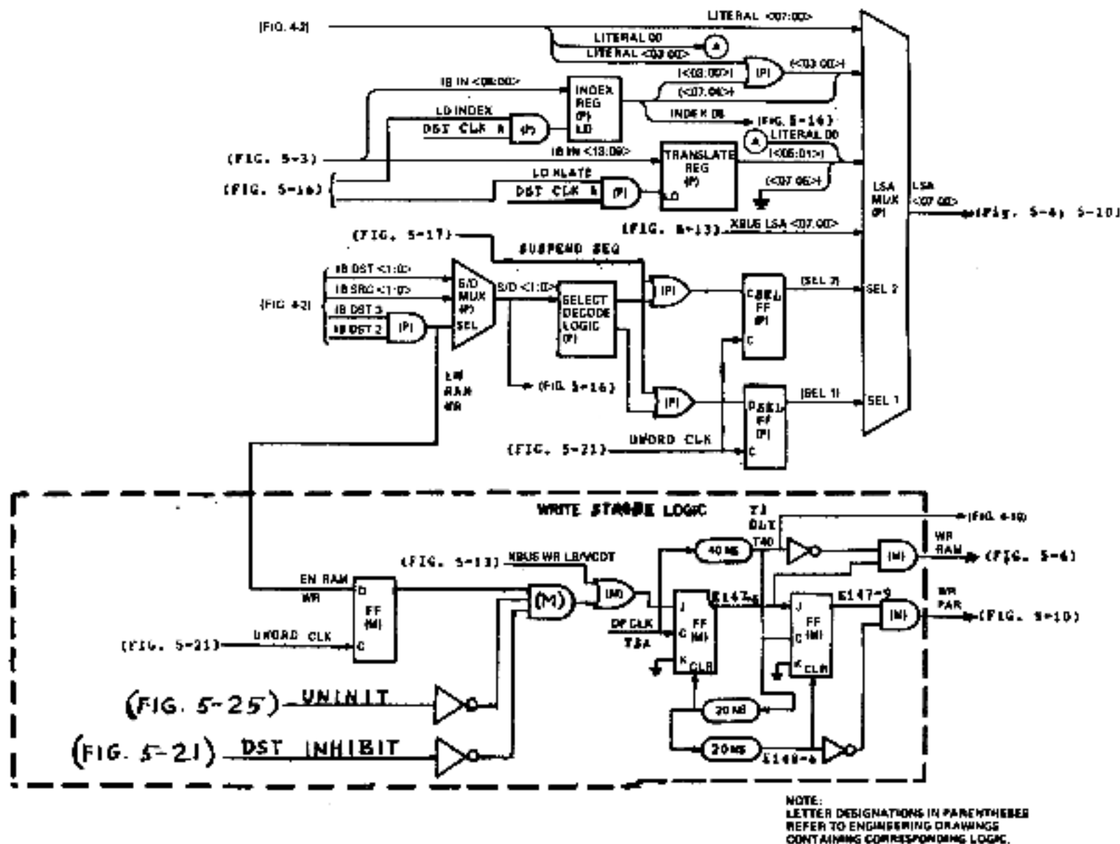
Figure 5-6 L6/VCDT Address Selection Block Diagram
