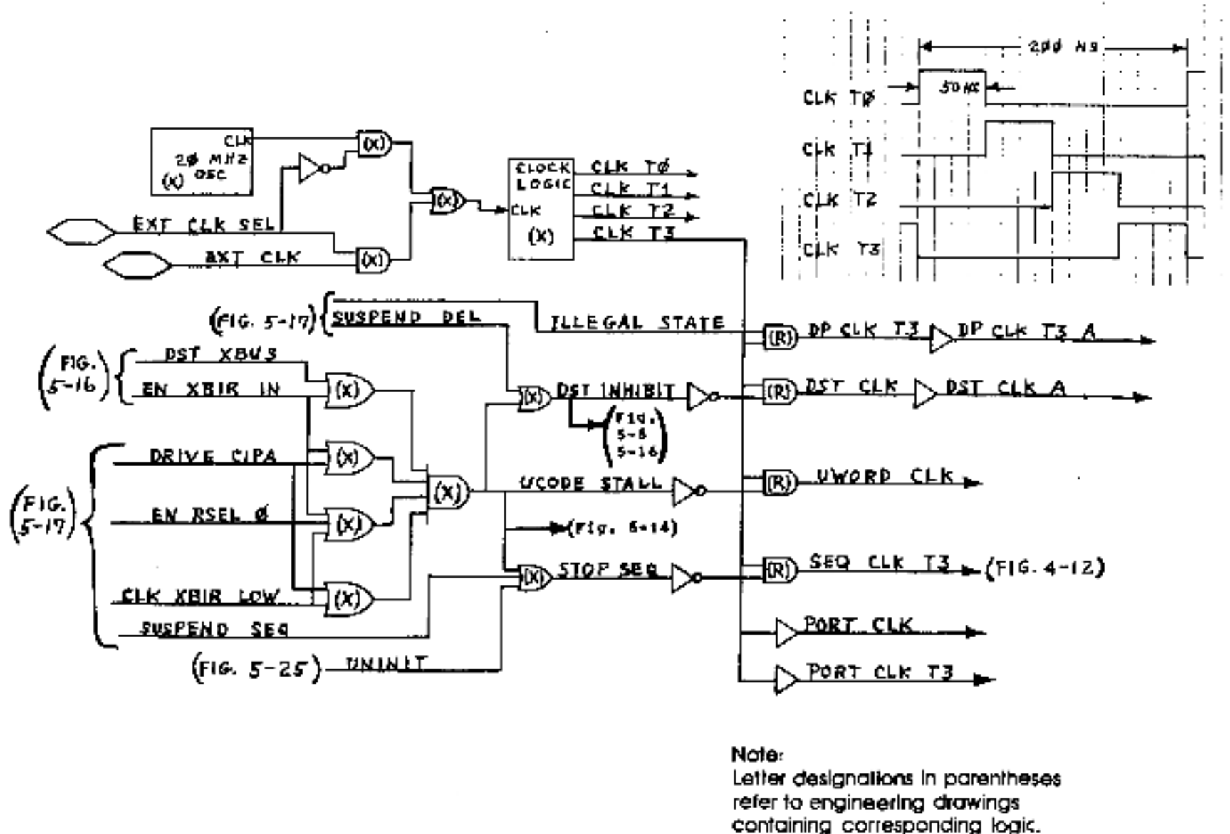
Figure 5-21 Port Clocks
