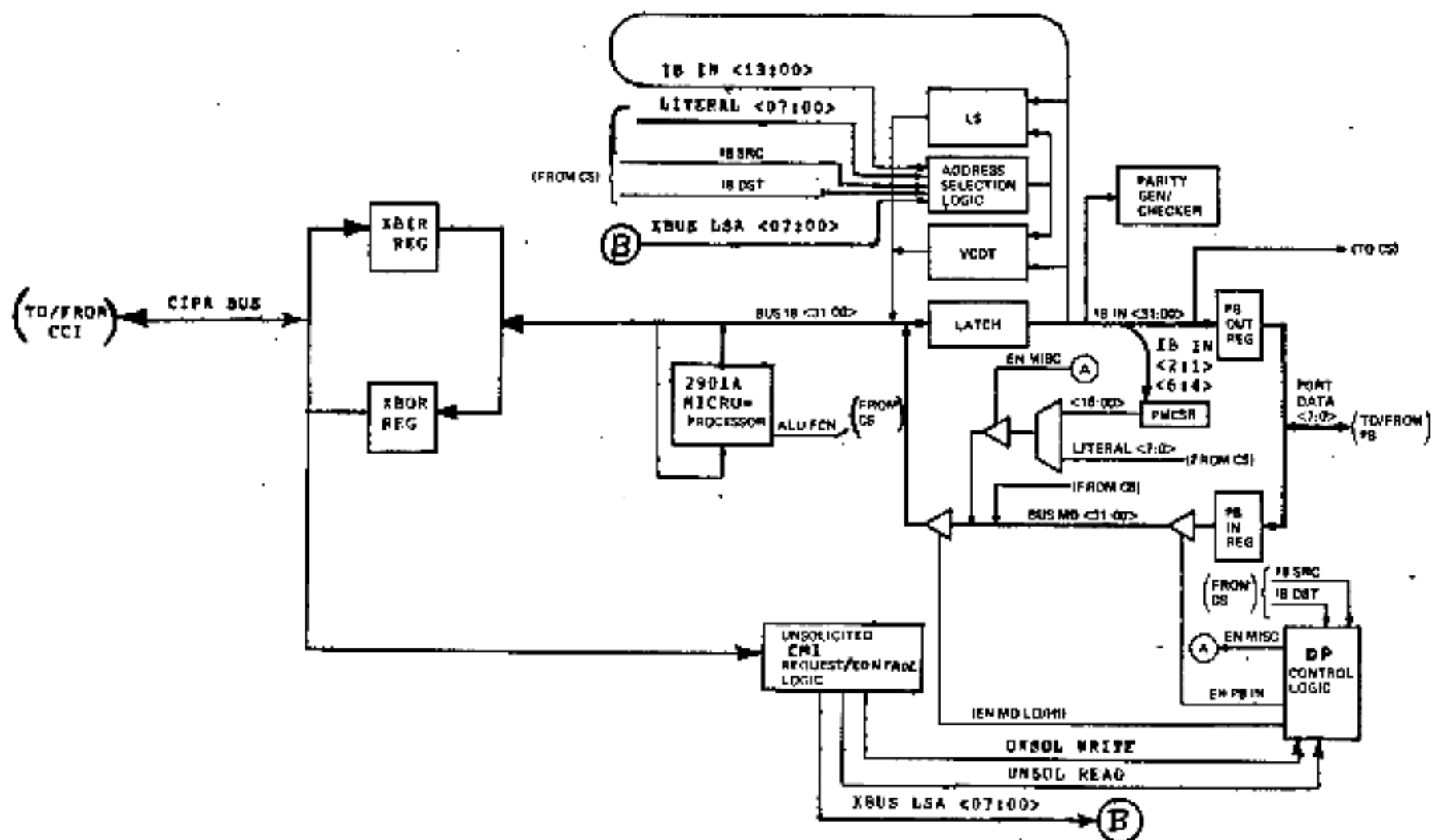
Figure 5-1 Data Path Module Block Diagram
