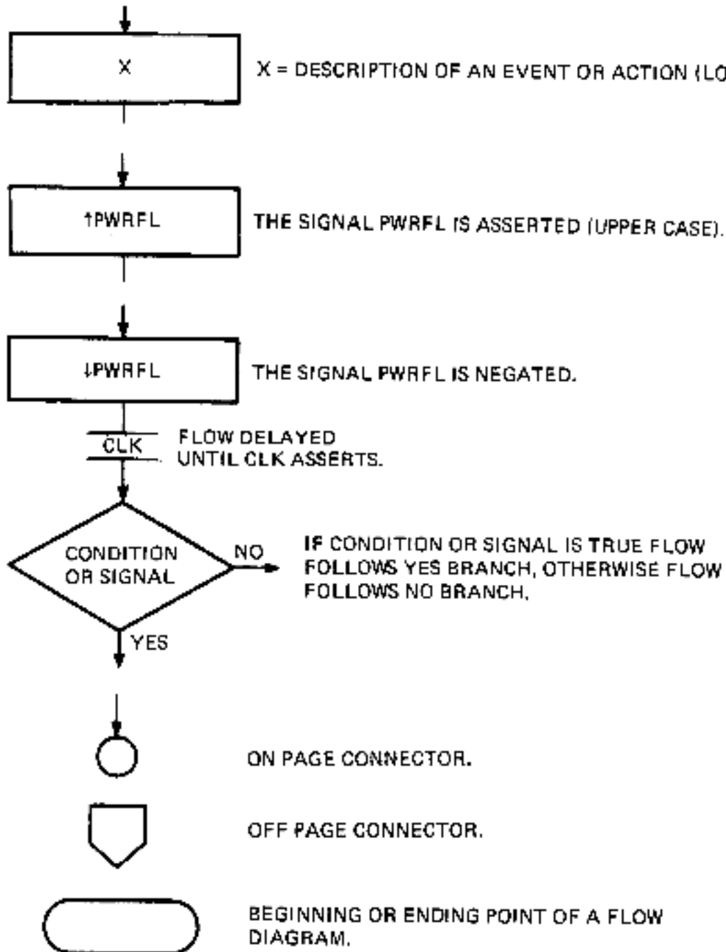
Figure B-1 Flow Diagram Symbols
