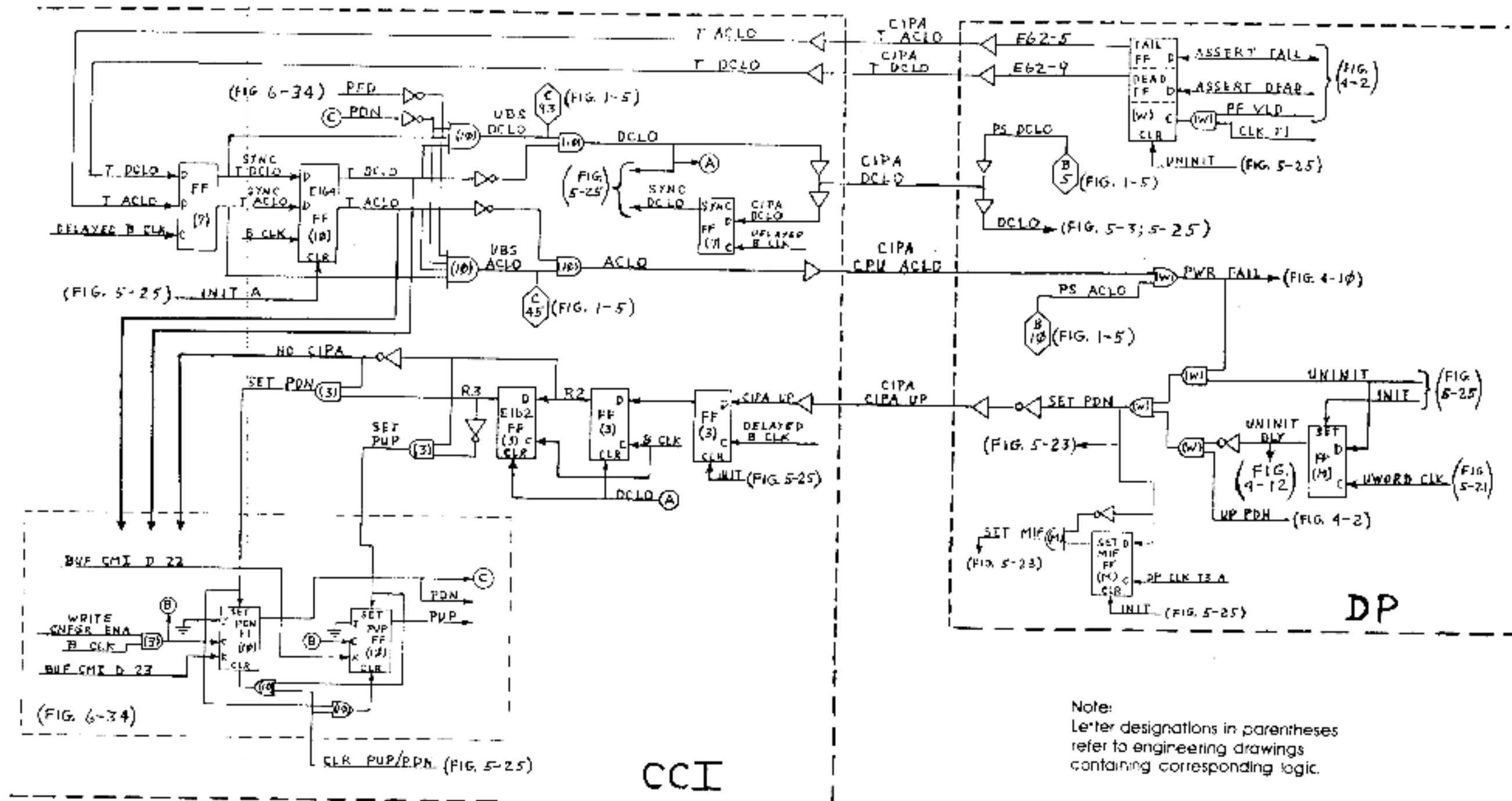
Figure 5-27 Power Control Logic
