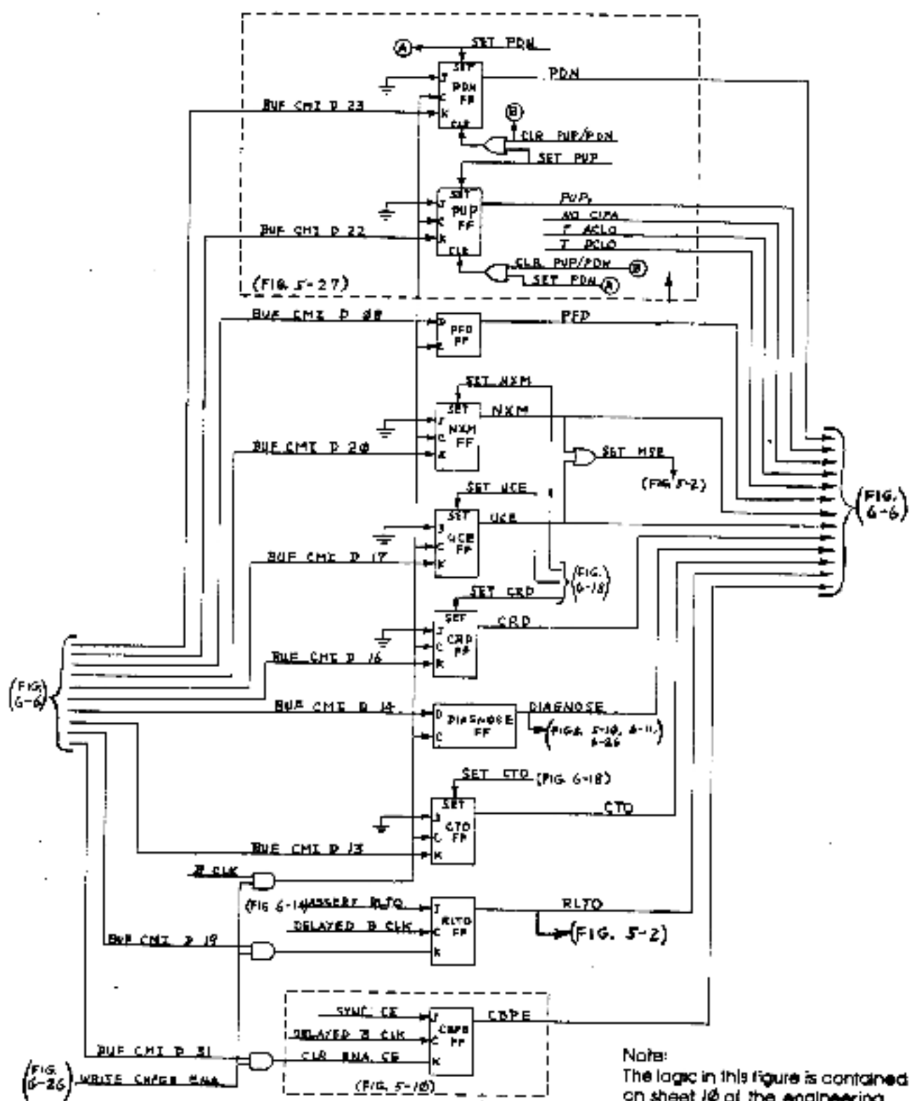
Figure 6-34 CNFR Register Logic
