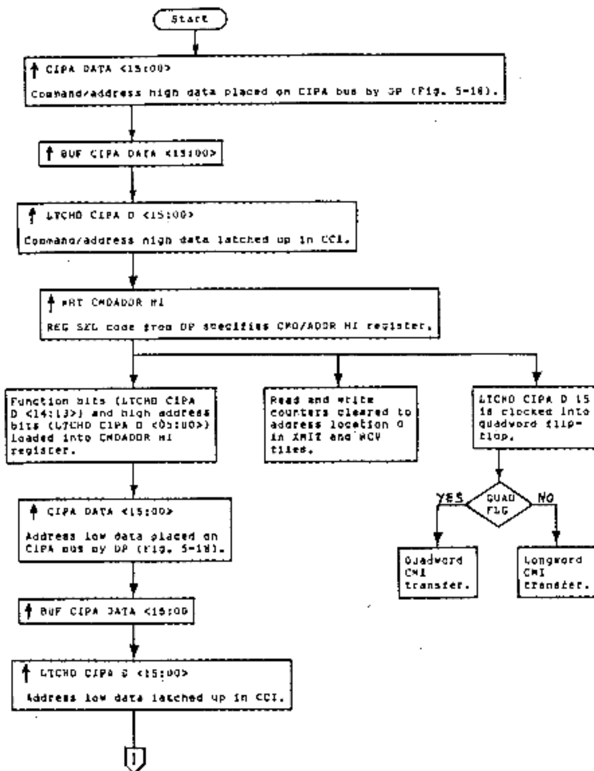
1 Figure 6-10 Load Flow Diagram for CMD/ADDR HI, ADDR LO, and Byte Mask Registers (Sheet 1 of 2)
