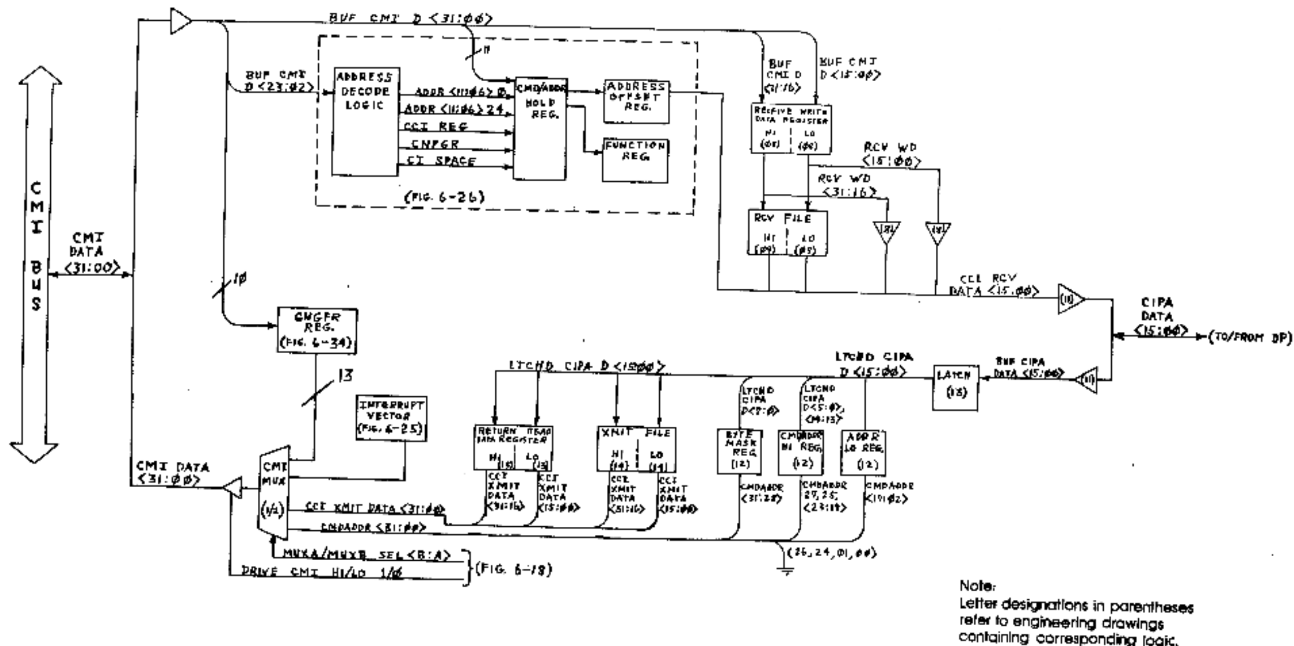
Figure 6-6 CCI Block Diagram
