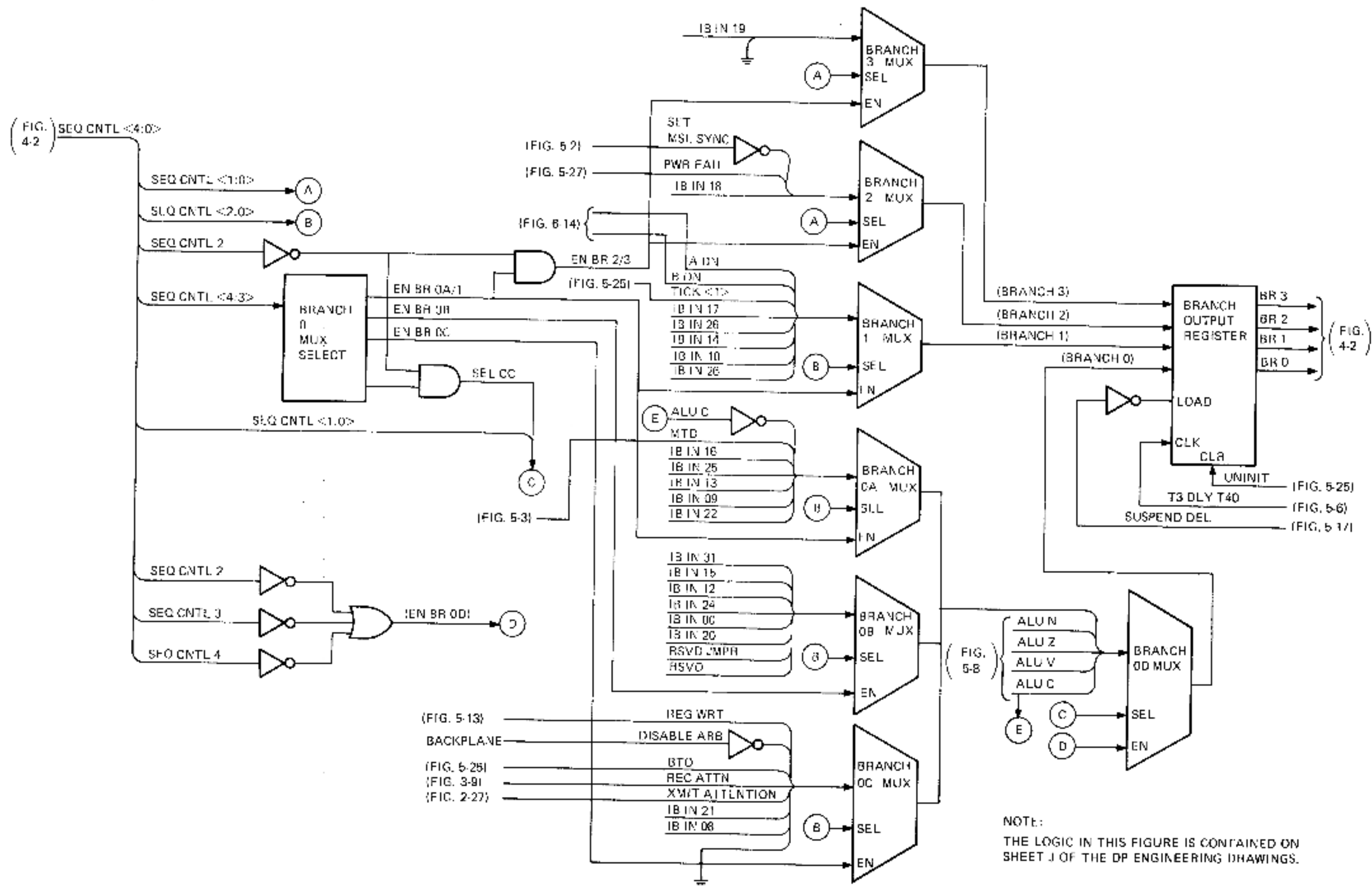
Figure 4-10 Branch Logic
