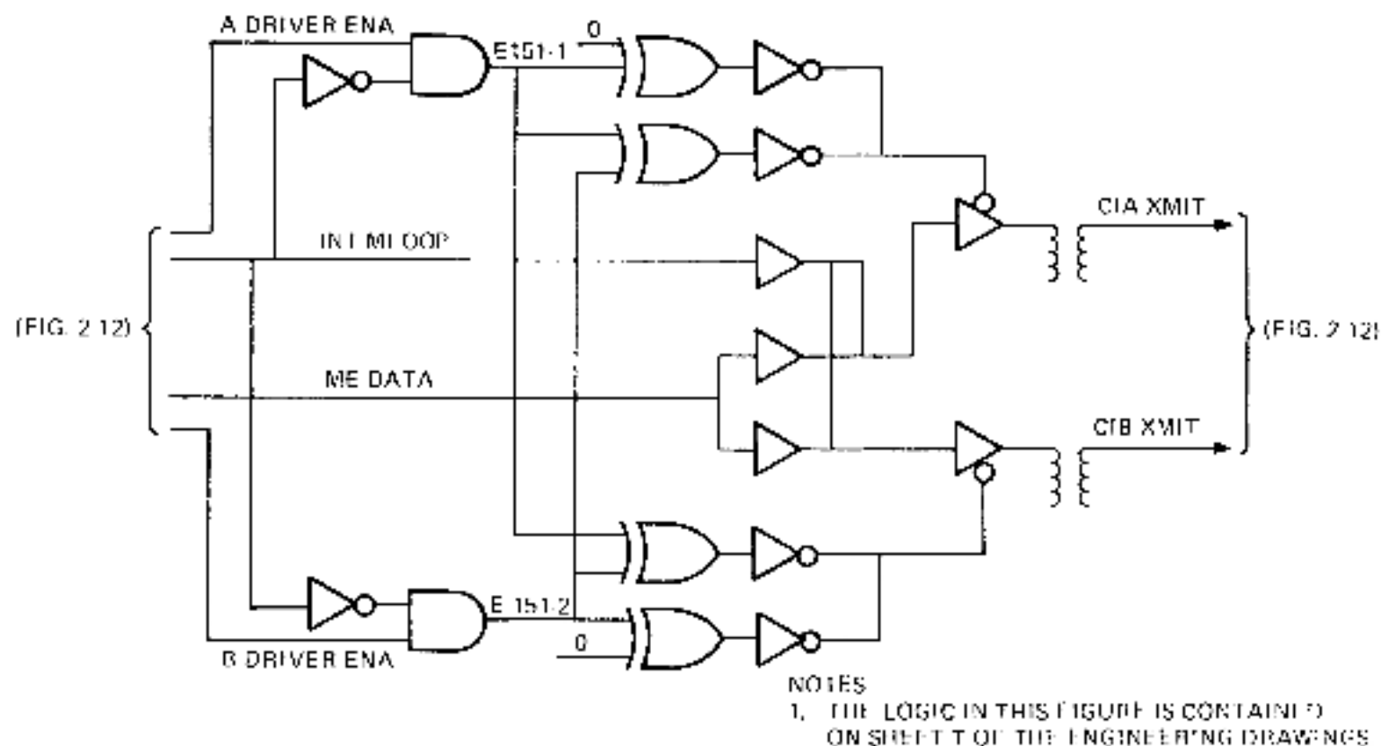
Figure 2-17 XMIT ECL Drivers
