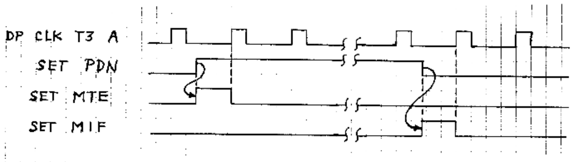
Figure 5-30 Power-Fail And Power-Up Interrupt Signals
