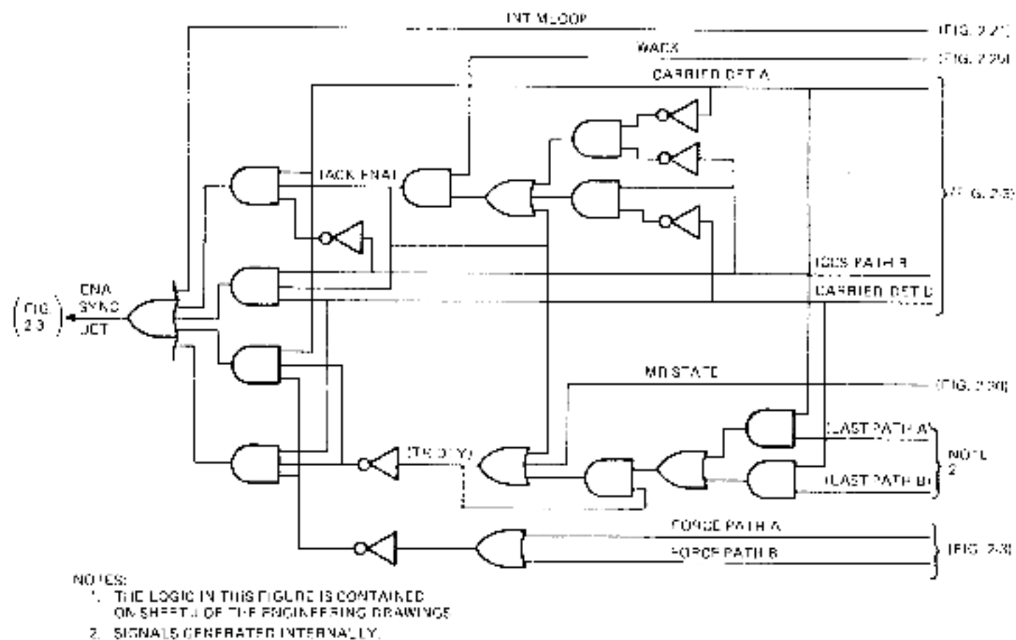
Figure 2-29 Sync Character Detect Enable PAL.
