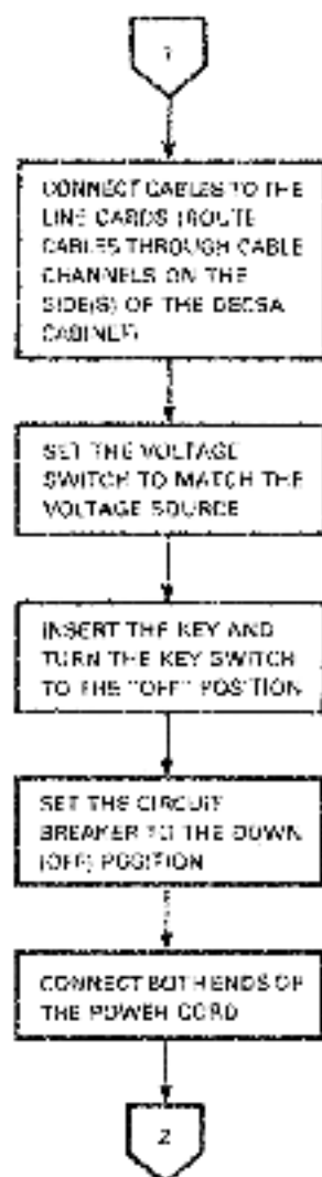
Figure 1 Installation Flow Diagram (Sheet 2 of 5)
