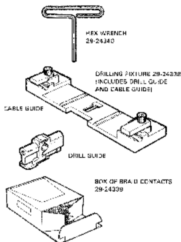
Figure 3 Transceiver Installation Kit Parts (Sheet 2 of 2)
