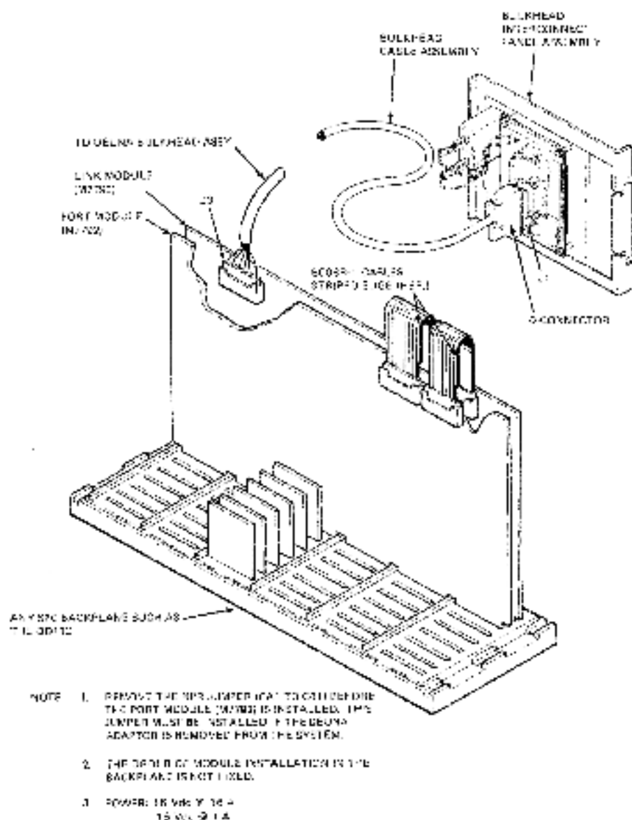
Figure 4 DEUNA Cabling Diagram
