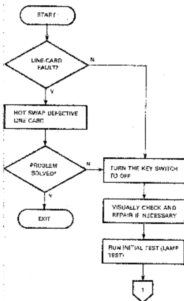
Figure 2 Troubleshooting Flow Diagram (Sheet 1 of 5)
