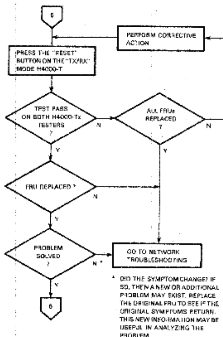
Figure 13 Troubleshooting Flow Diagram (Sheet 6 of 7)
