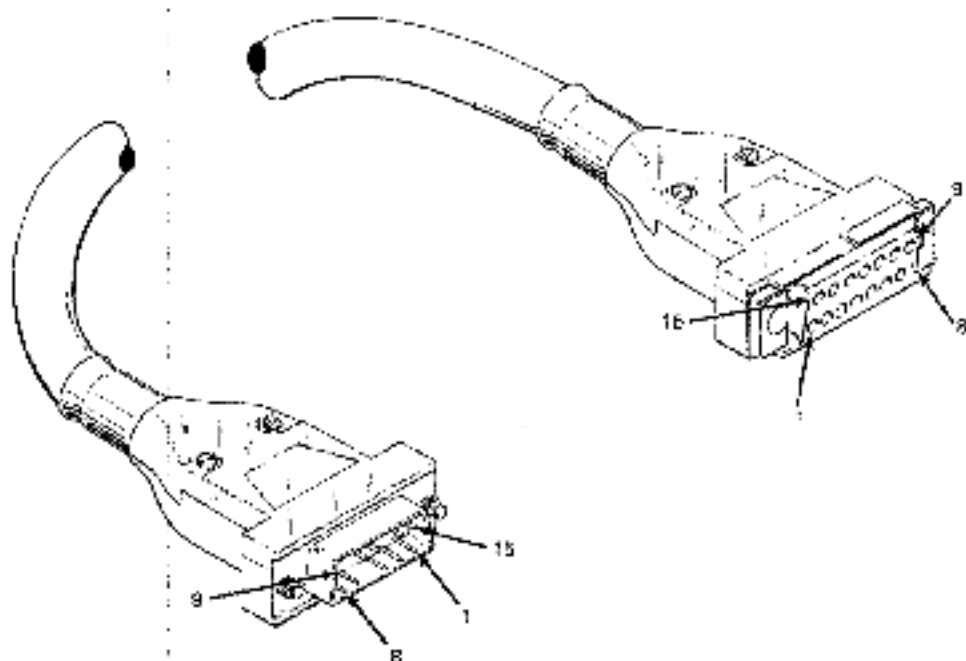
Figure 6 BNE3A-**-BNE4A-** (PVC) and BNE3B-**-BNE4B-** (Teflon ® ) Transceiver Cables
