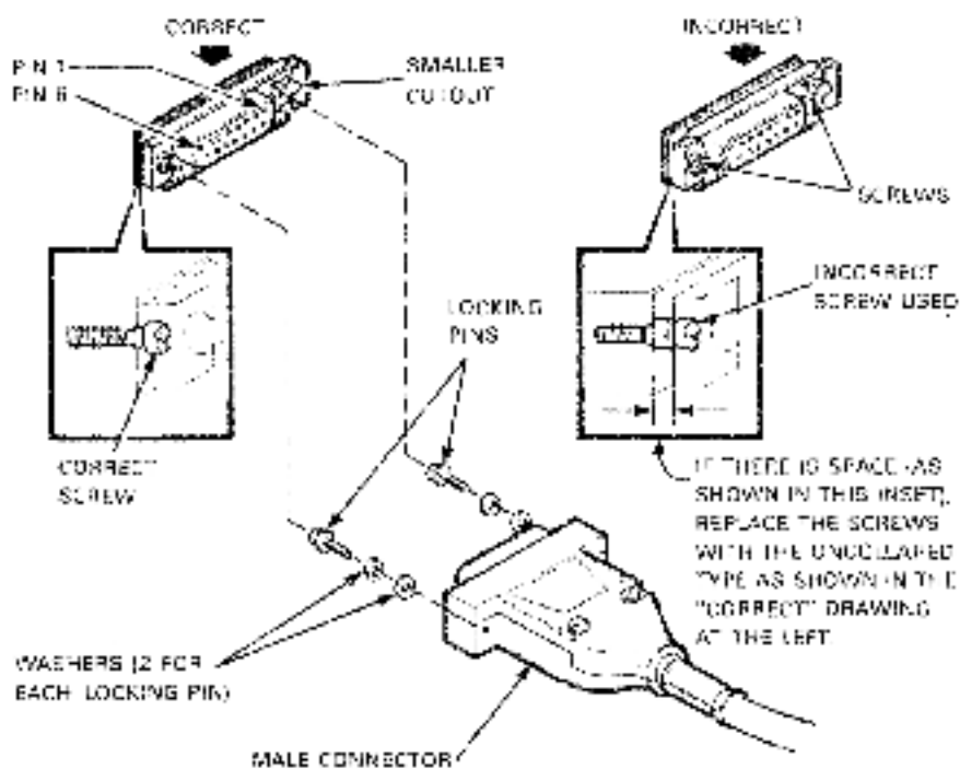
Figure 17 Proper Slide-Latch Configuration
