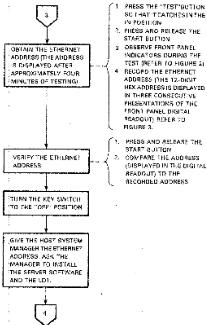
Figure 1 Installation Flow Diagram (Sheet 4 of 5)
