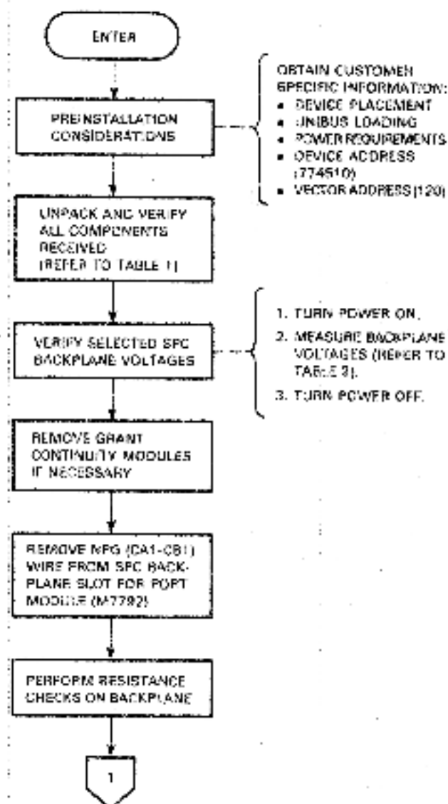
Figure 1 Installation Flow Diagram (Sheet 1 of 5)
