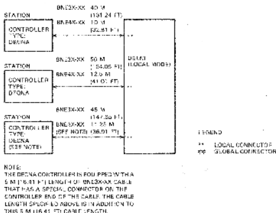
Figure 9 Maximum Cable Lengths with Single-Tier DELNI LAN
