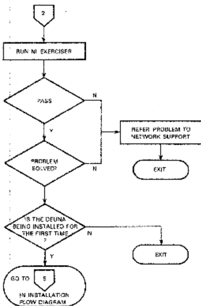
Figure 9 DEUNA Troubleshooting Flow Diagram (Sheet 3 of 3)
