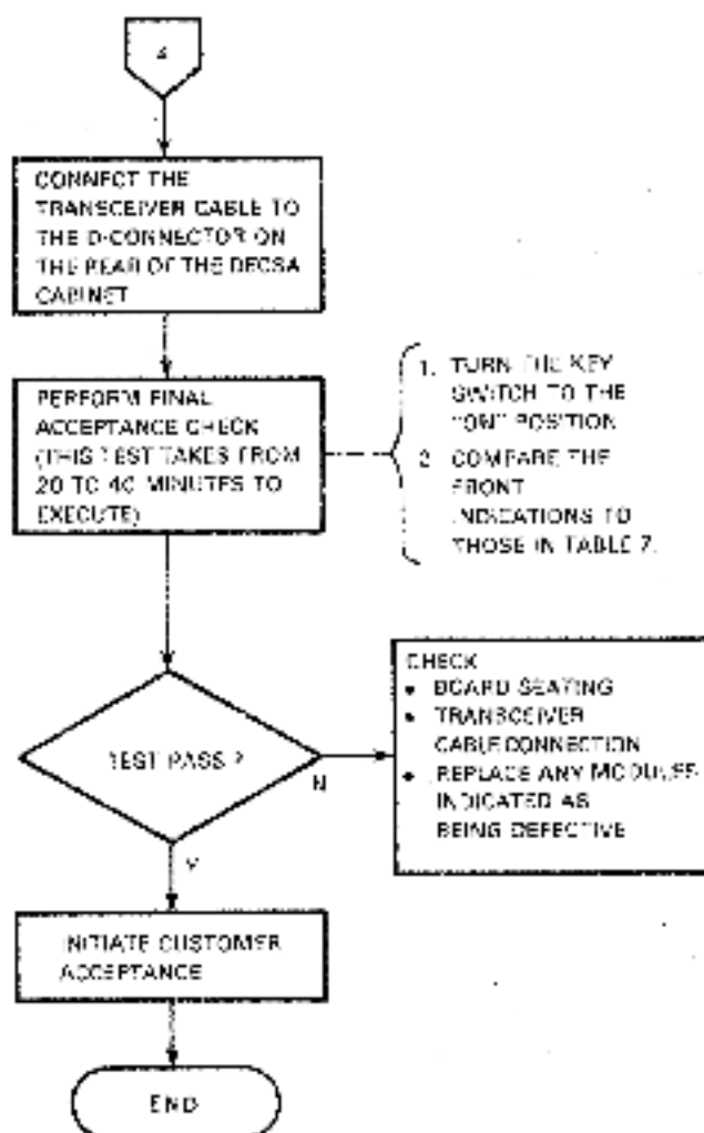
Figure 1 Installation Flow Diagram (Sheet 3 of 5)
