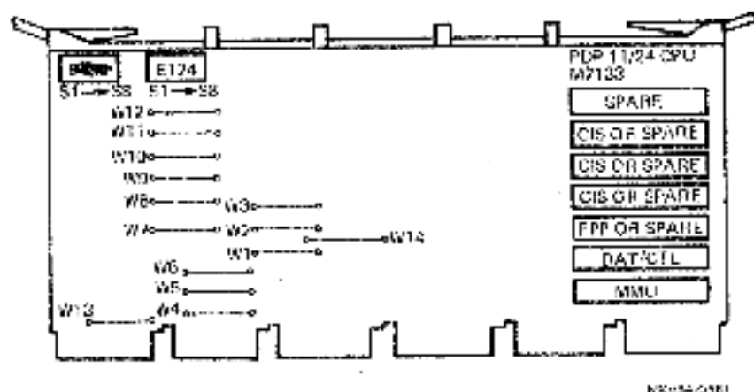
Figure 8 M7133 (PDP-11/24) CPU Switch and Jumper Locations
