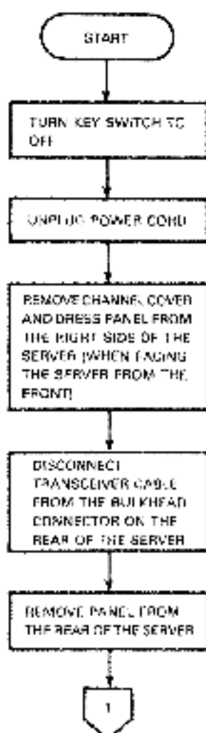
Figure 10 Upgrade: Adding a Second PAM Set and Power Supply (Sheet 1 of 5)
