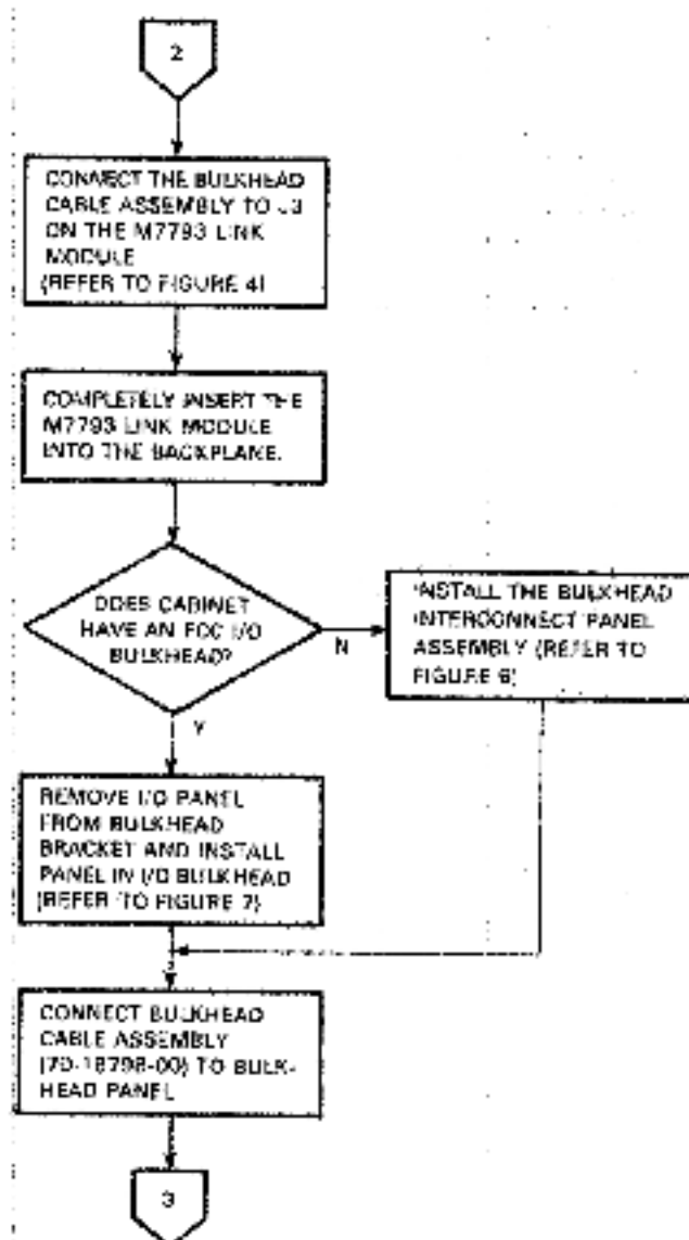
Figure 1 Installation Flow Diagram (Sheet 3 of 5)
