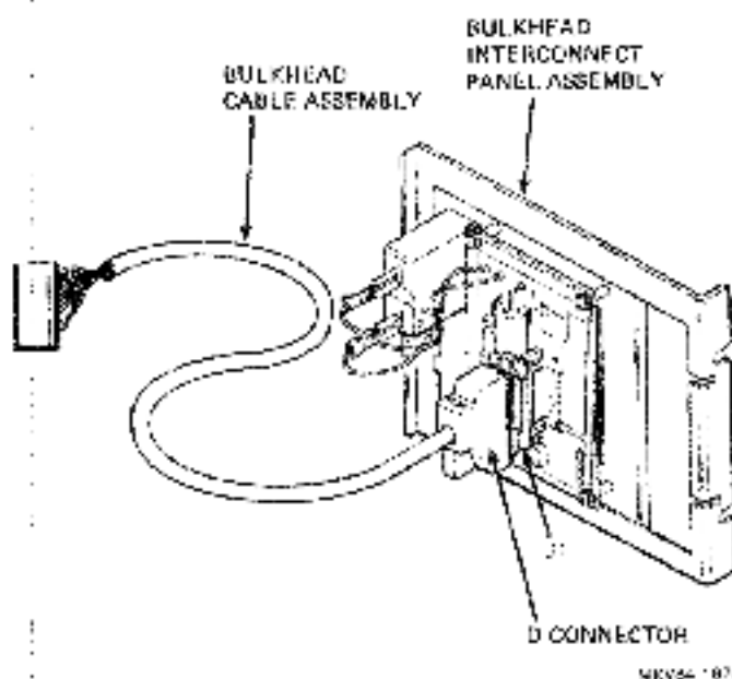
Figure 16 70-18798-01 Bulkhead Cable Assembly and 70-18799-00 Bulkhead Interconnect Panel Assembly
