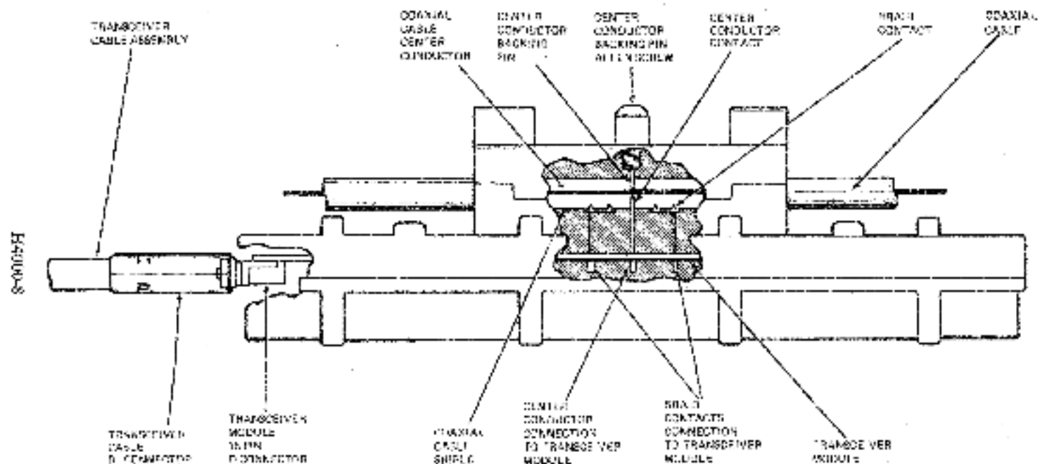
Figure 4 H4000 Ethernet Transceiver: Cutaway View Showing Coaxial Cable Interface.
