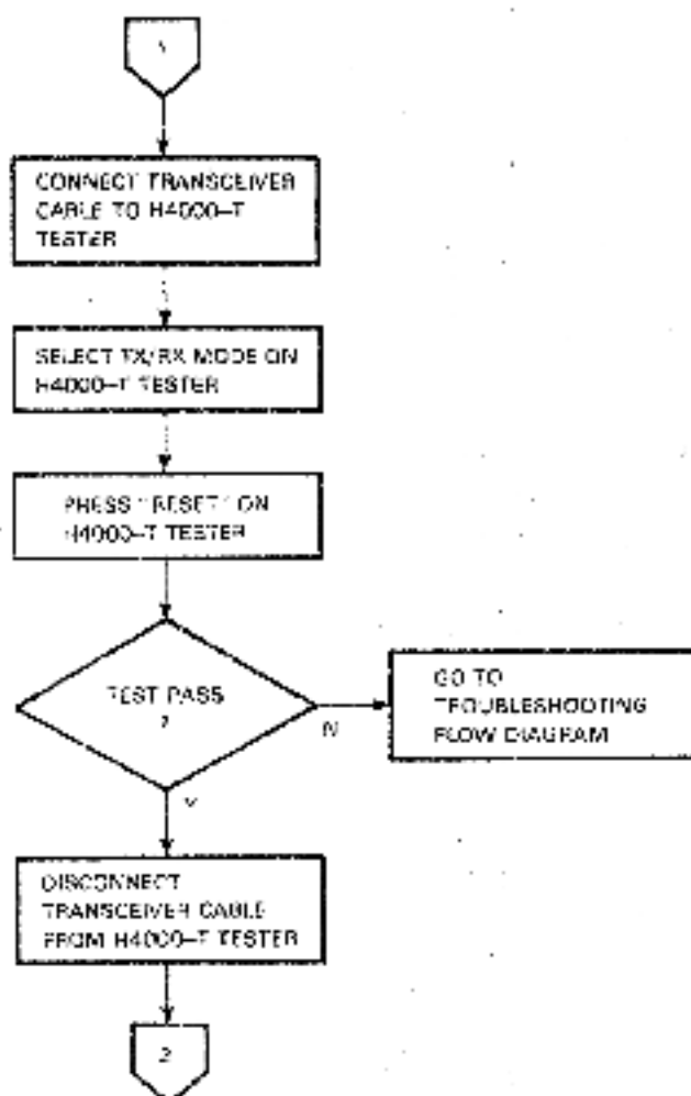
Figure 2 Installation Flow Diagram (Sheet 2 of 4)
