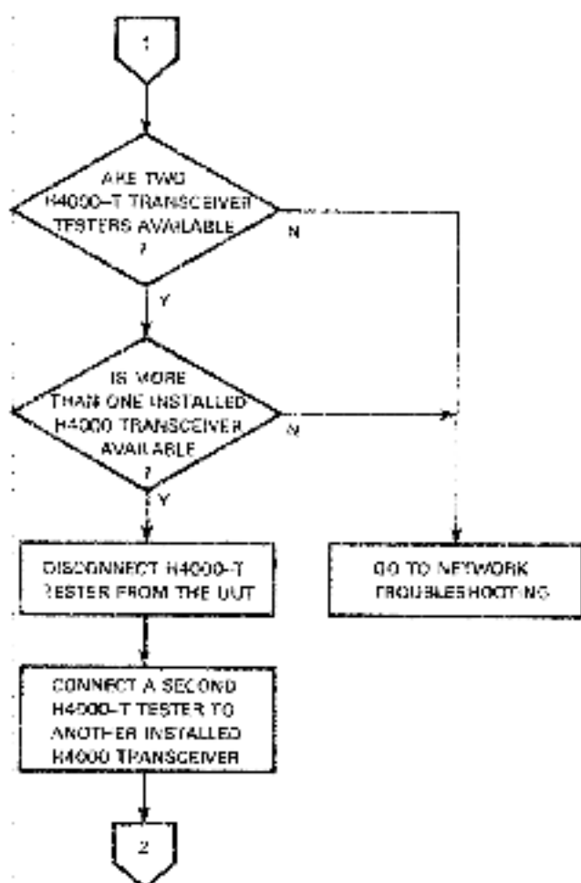
Figure 6 Troubleshooting Flow Diagram (Sheet 2 of 4)
