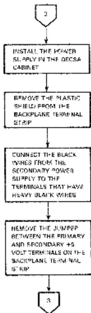
Figure 10 Upgrades: Adding a Second PAM Sol and Power Supply (Sheet 3 of 5)
