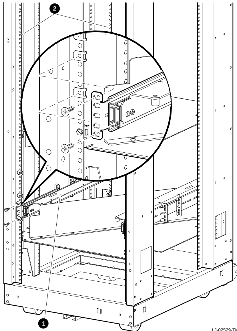
Figure 2-7 Installing the Left Side Chassis Slide Assembly
