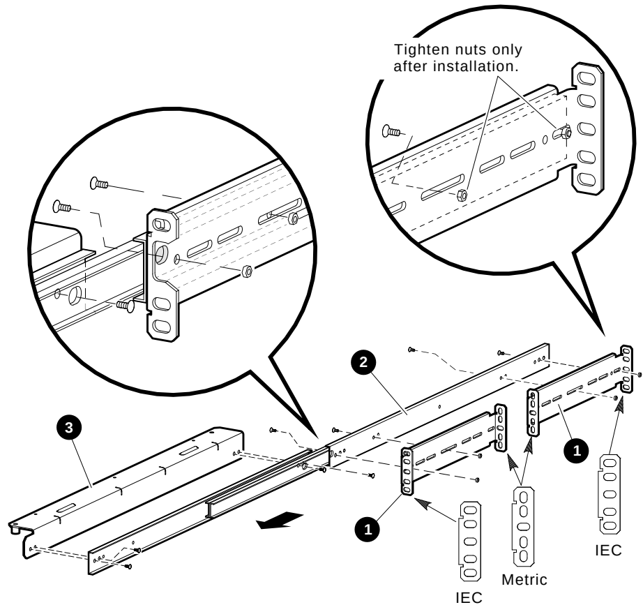
Figure 1-4 Assembling the Right Side Chassis Slide Subassembly
