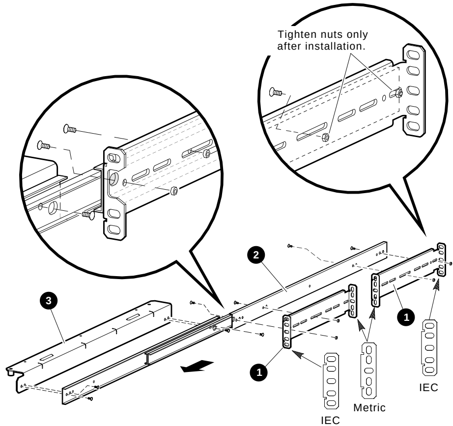
Figure 2-4 Assembling the Right Side Chassis Subassembly
