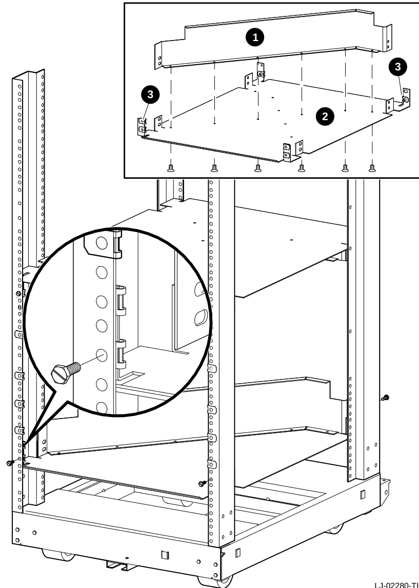
Figure 1-3 Installing the Bottom Air Deflector Assembly
