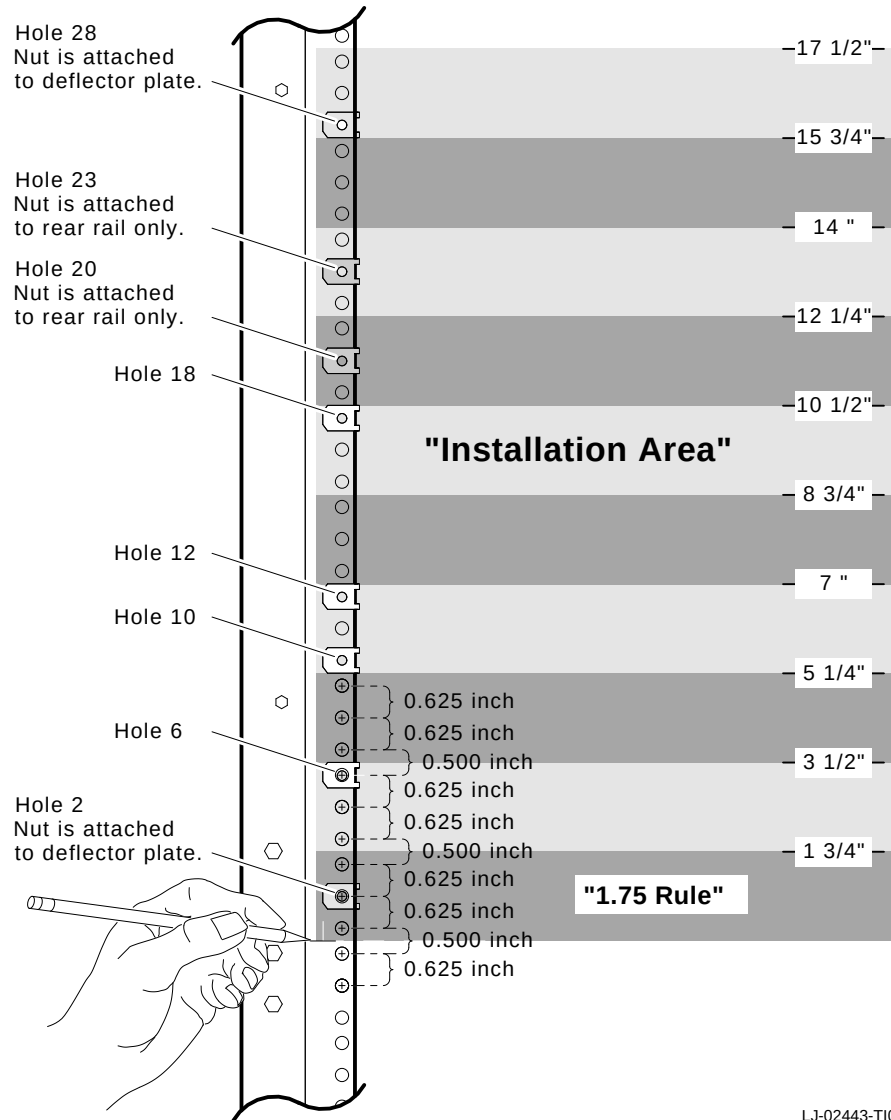
Figure 2-1 Determining the Installation Area
