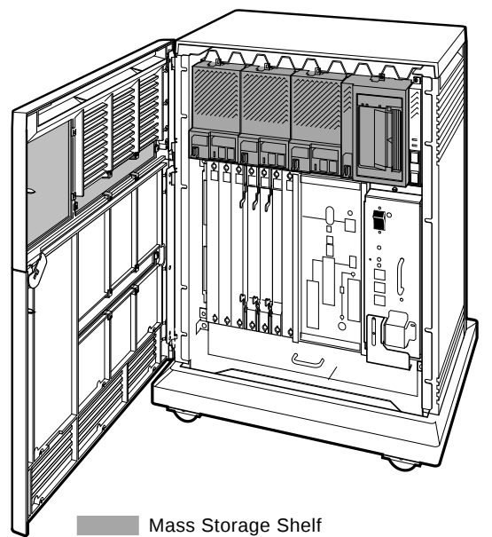
Figure 9-2 Mass Storage Shelf
