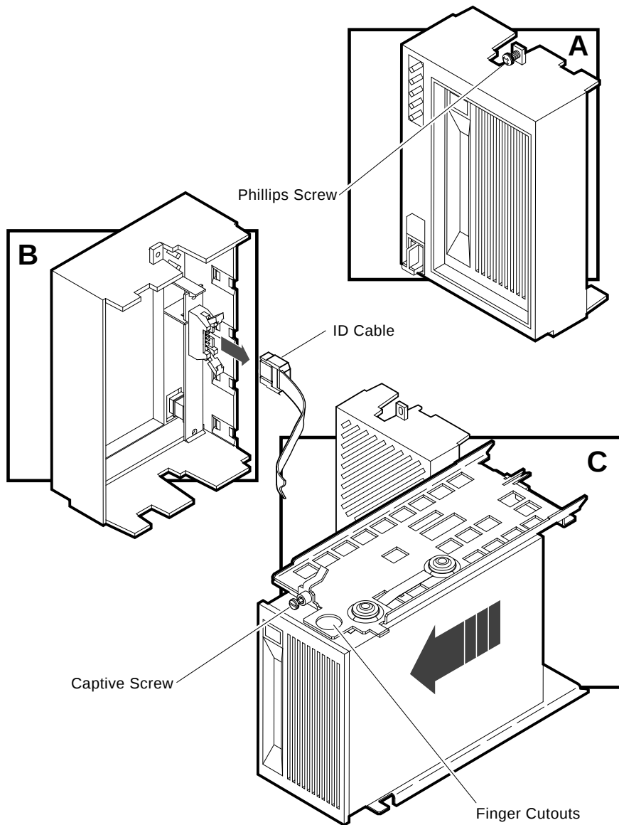
Figure 9-9 Remove the TLZ04 Tape Drive
