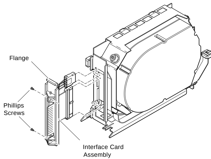
Figure 9-7 Disconnect Cables
