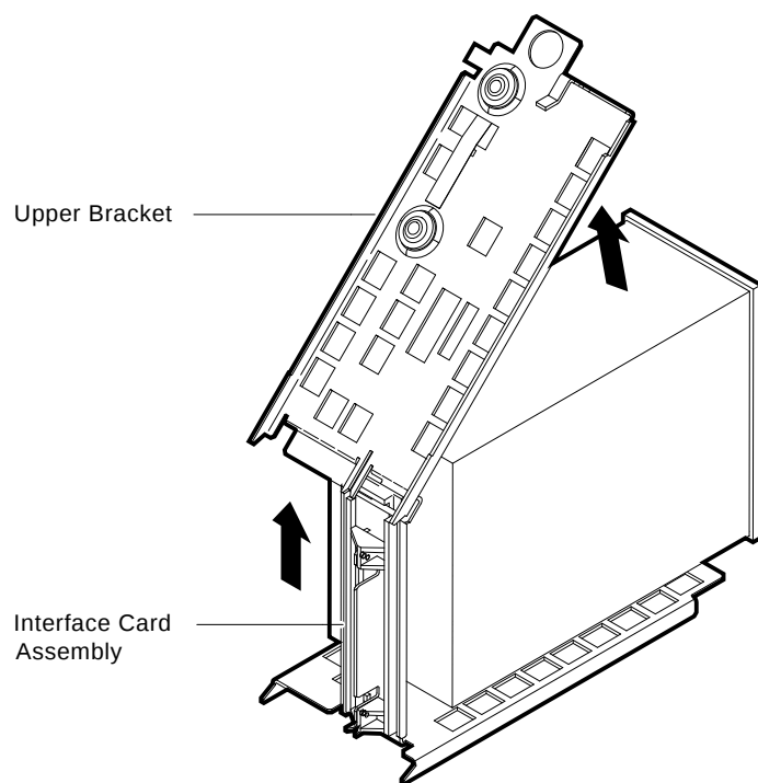
Figure 9-11 Remove the Drive Top Mounting Bracket
