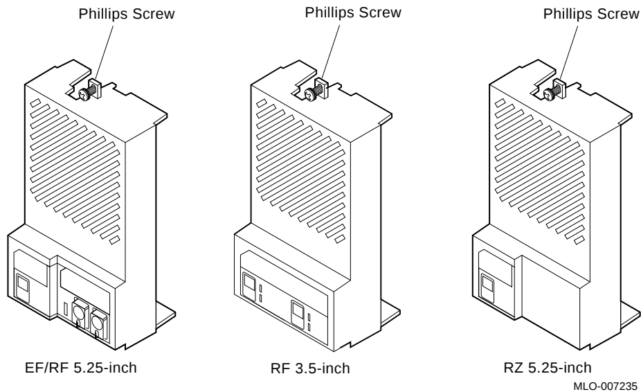
Figure 9-3 Front Panel Assemblies
