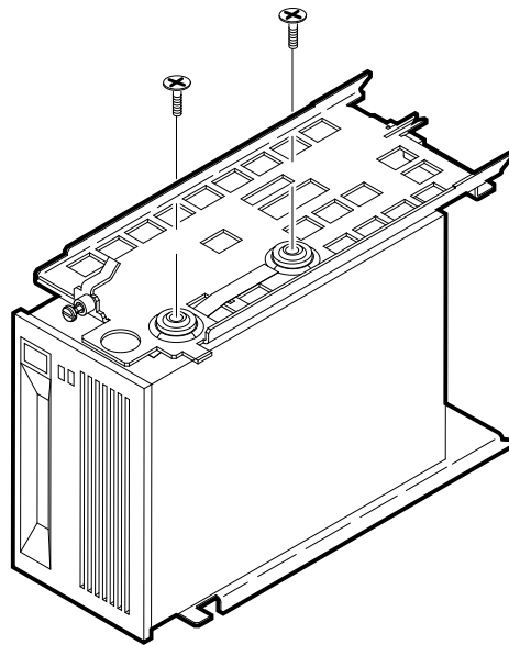
Figure 9-10 Remove Bracket Screws
