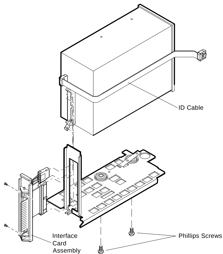
Figure 9-13 Remove the Bottom Bracket
