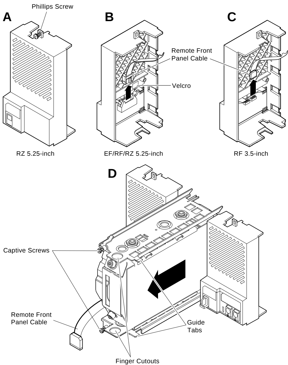
Figure 9-4 Remove RZ56E
