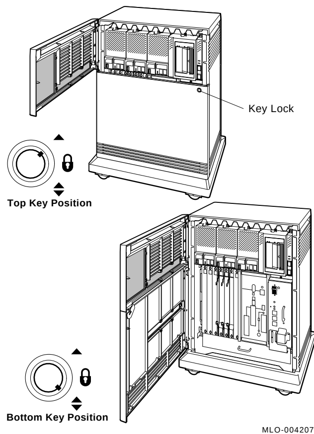
Figure 9-1 Keylock Positions
