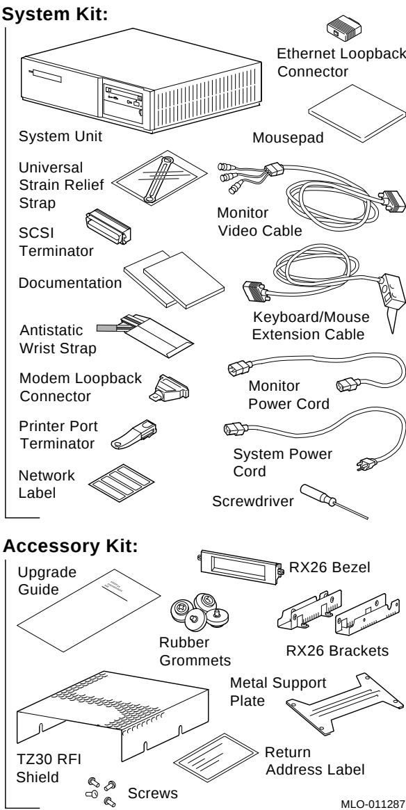
Figure 1-1 Upgrade Kit Contents
