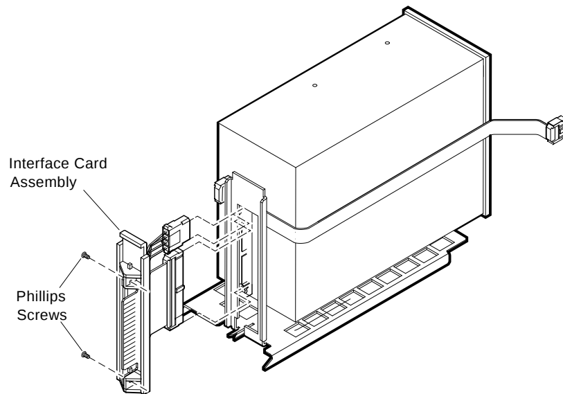
Figure 9-12 Disconnect Cables
