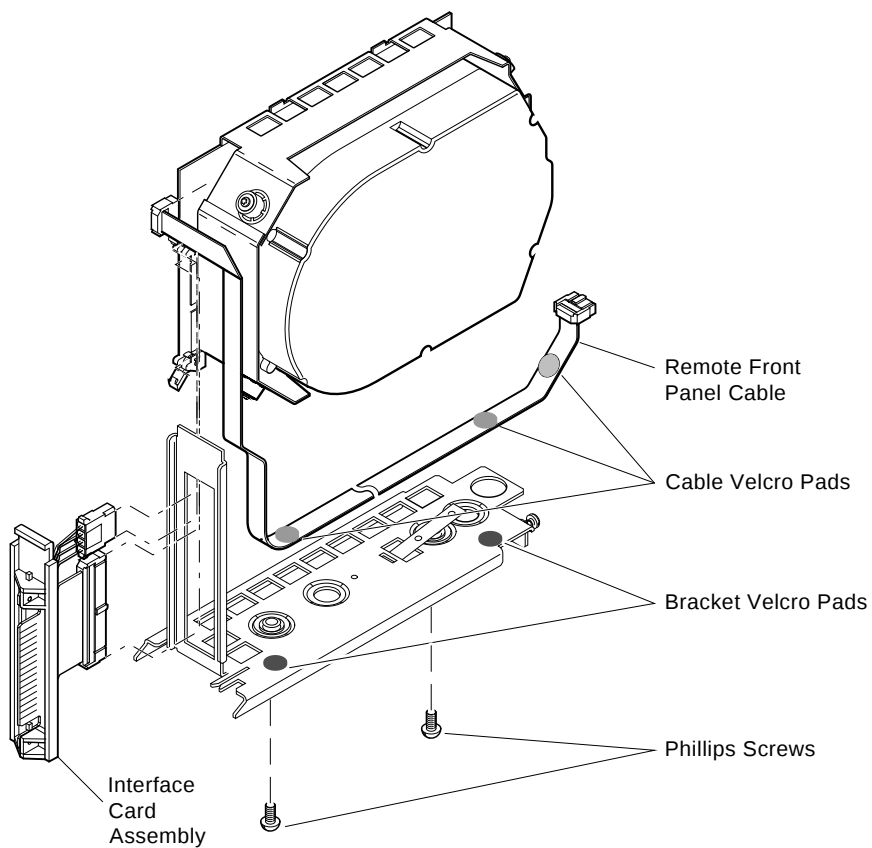
Figure 9-8 Remove the Bottom Bracket
