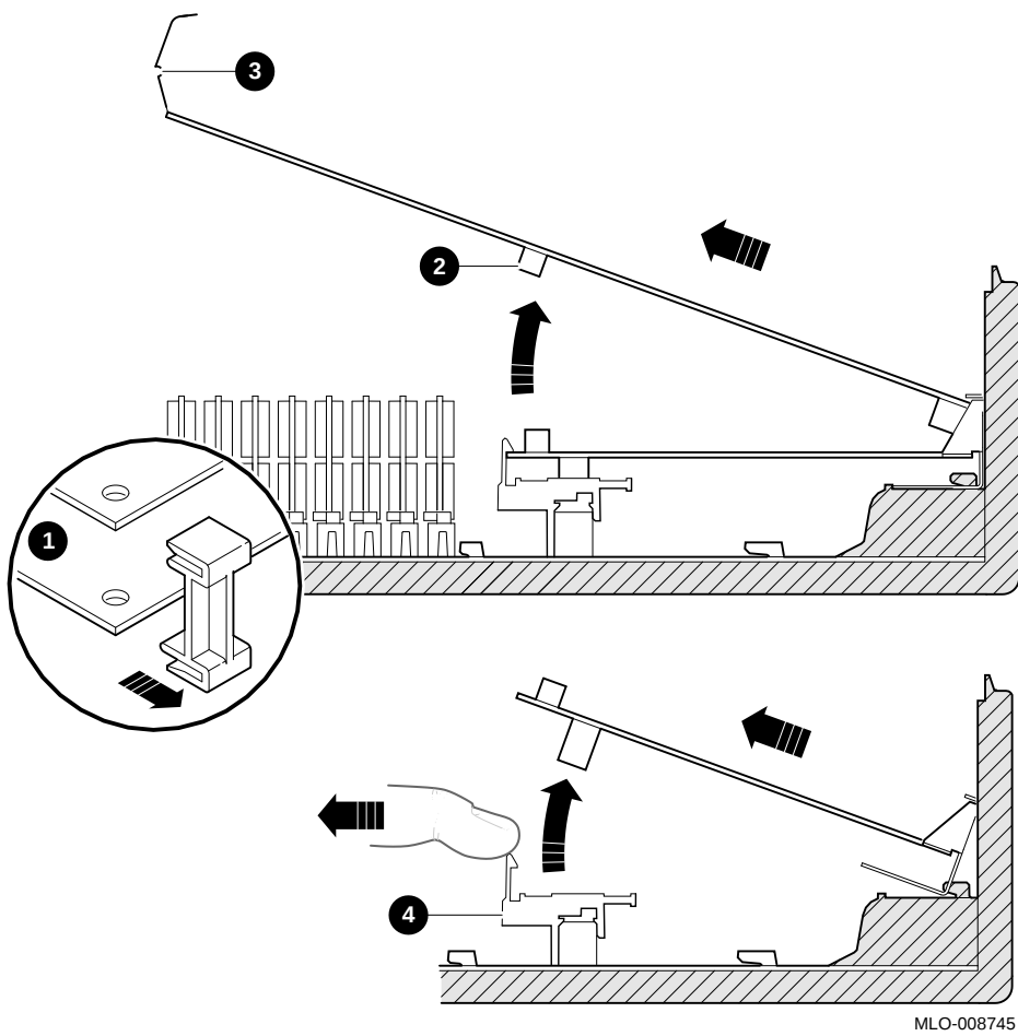
Figure 4-2 Removing the SPXgt 24-Plane Graphics Module
