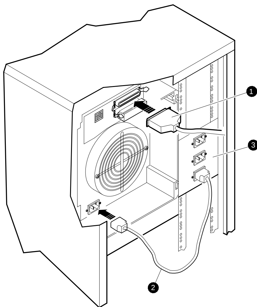
Figure 4-65 Disconnecting/Connecting a TZ857
