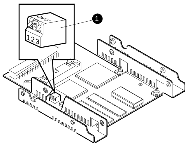
Figure 4-43 SCSI ID Switches on an RX26
