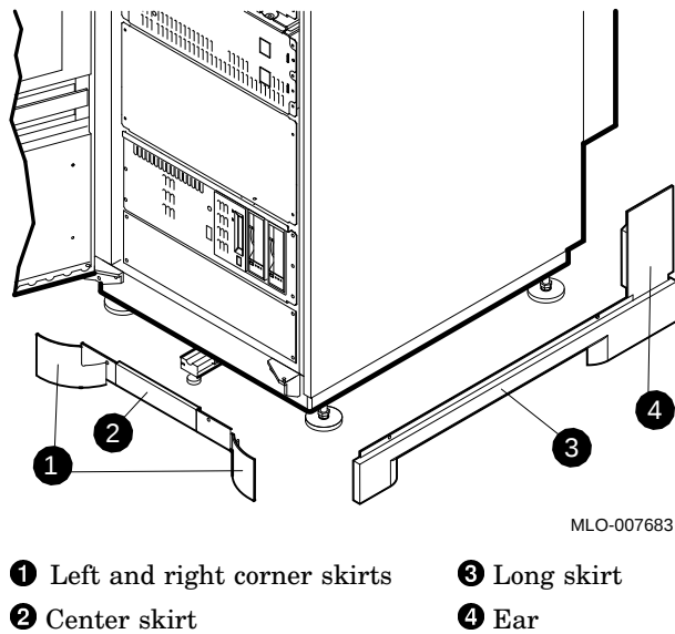
Figure 2-4 Front and Side Skirts
