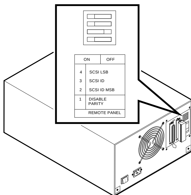
Figure 4-64 SCSI ID Switches on an External TZ85
