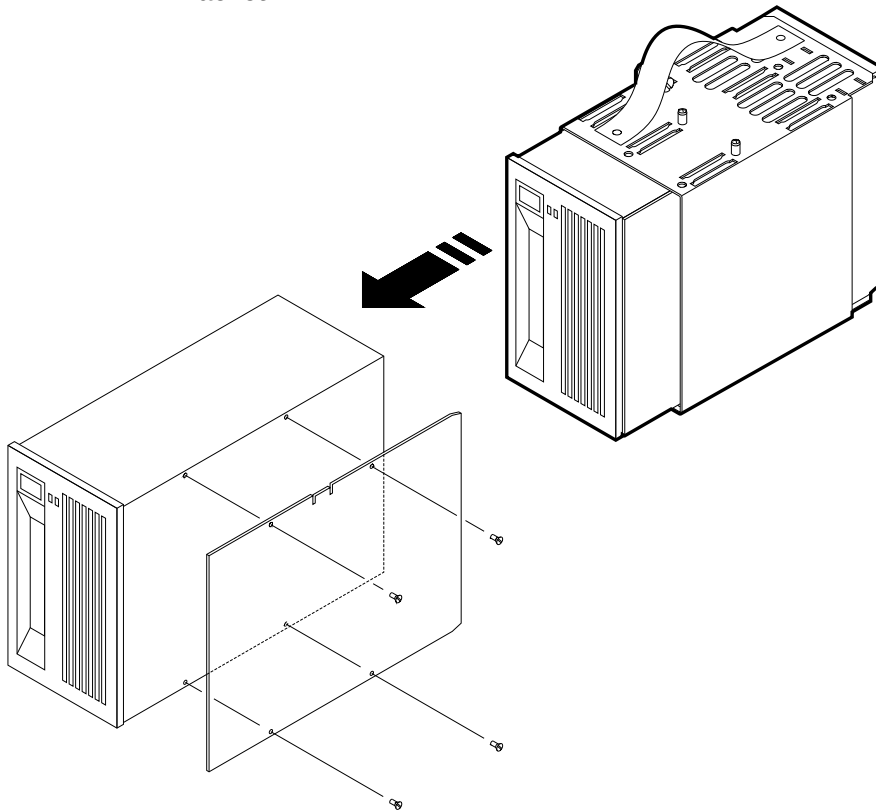
Figure 4-13 Removing a Full-Height Device from a Removable Media Device Bracket
