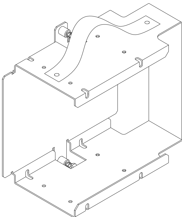
Figure 4-6 Drive Bracket
