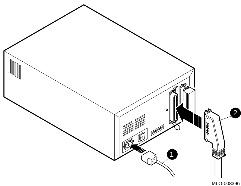
Figure 4-60 Disconnecting/Connecting an External TKZ09
