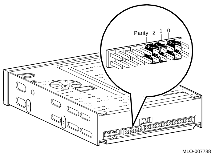
Figure 4–55 SCSI ID Jumpers on a TZK10
