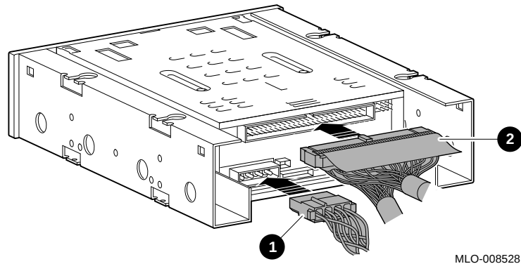
Figure 6–7 Connecting Cables to the TLZ06 Drive
