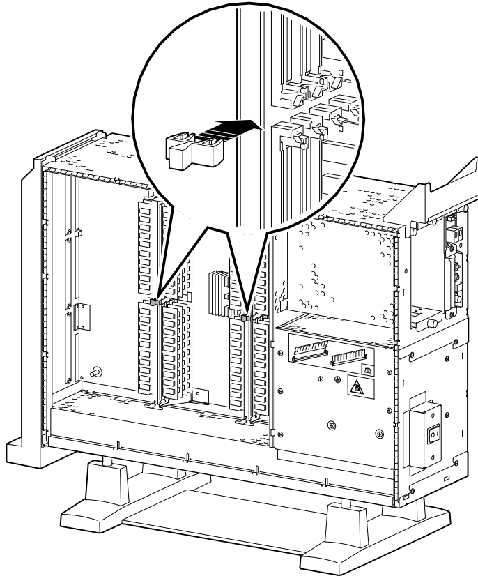
Figure 9–10 Installing MMB Clips
