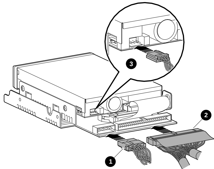
Figure 4-8 Connecting Cables to the RX26 Drive
