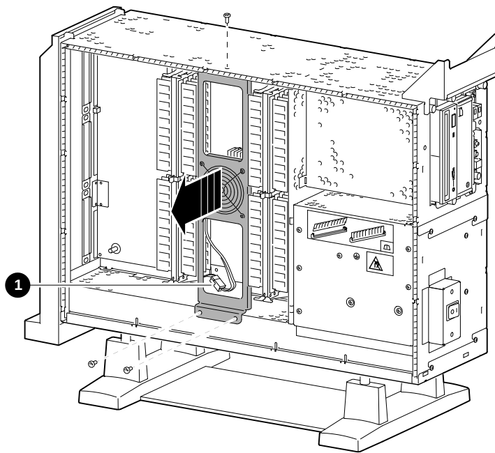
Figure 9-12 Removing the Fan Bracket
