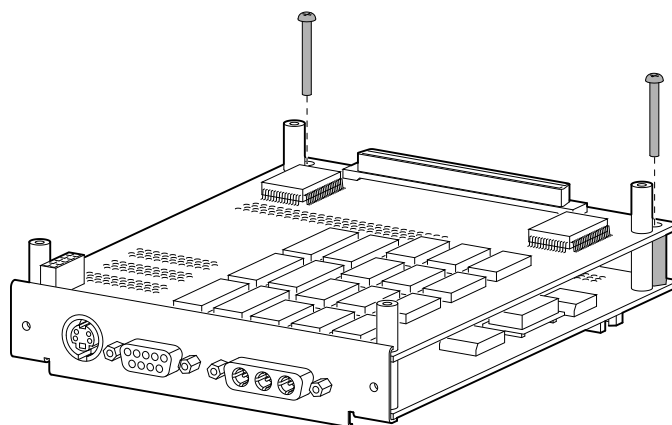
Figure 10–12 TX Module Modification
