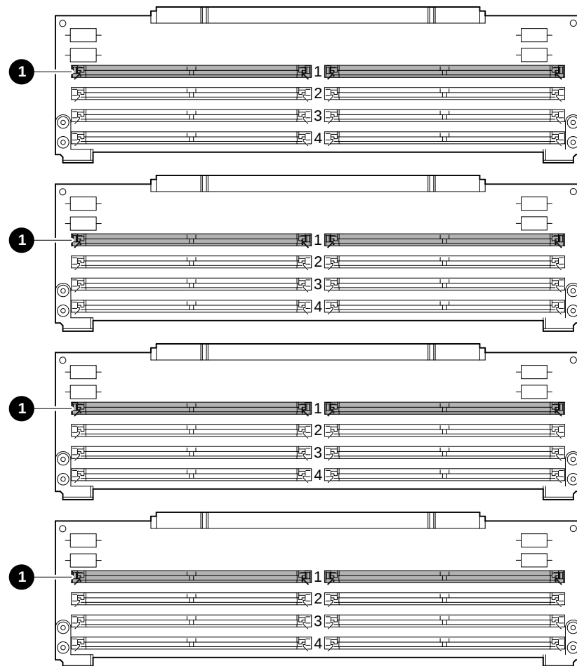
Figure 9–7 Placing the MMBs
