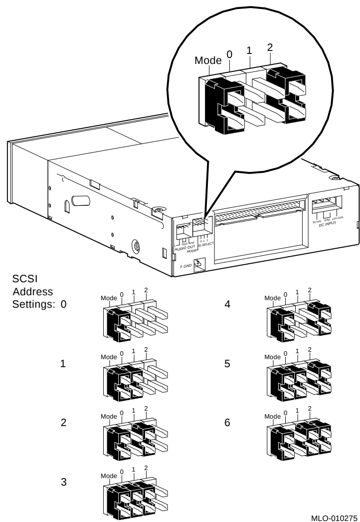
Figure 3-2 RRD42 Mode and SCSI Address Jumpers
