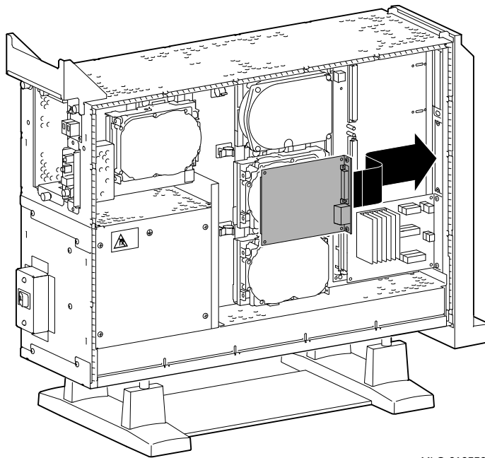
Figure 10–15 Seating a TURBOchannel Module
