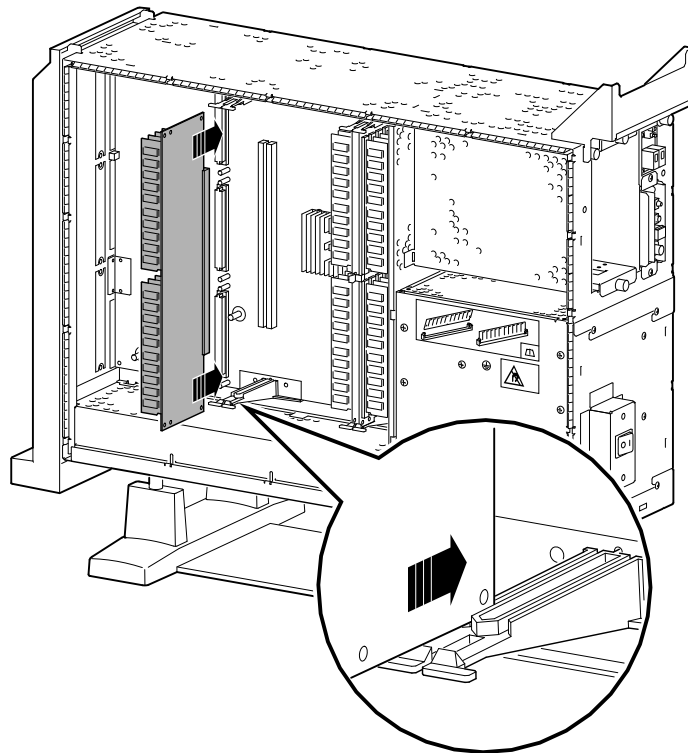
Figure 9–16 Installing an MMB
