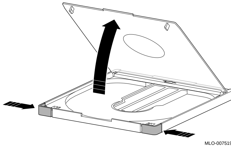
Figure 3–16 Opening the Compact Disc Caddy
