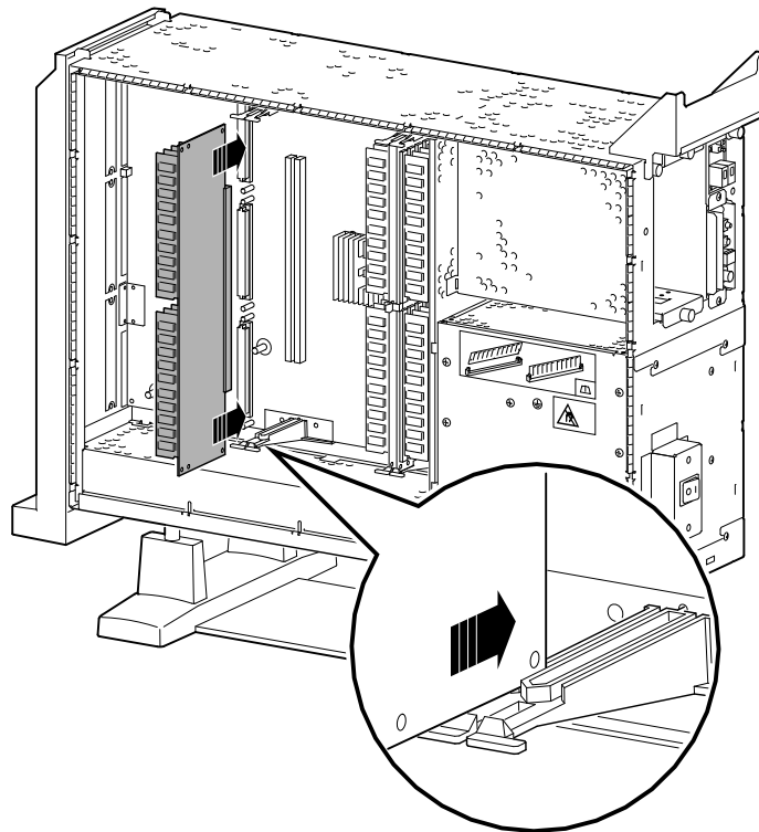
Figure 9–9 Installing an MMB
