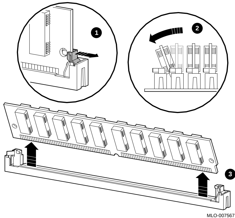
Figure 9-15 Removing a Memory Module
