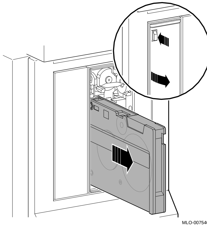
Figure 5-17 Removing the TZK10 Tape Cartridge
