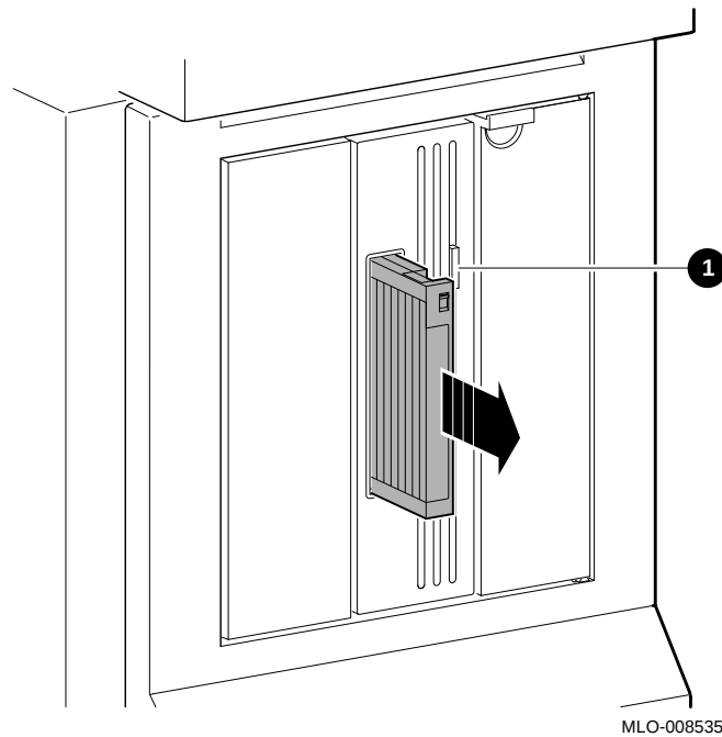
Figure 6–18 Removing the TLZ06 Tape Cassette
