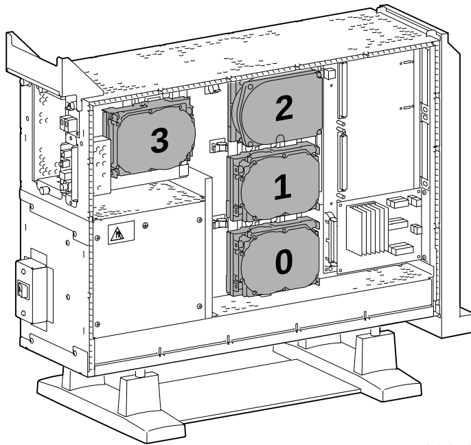
Figure 8–3 Fixed Disk Drive Positions
