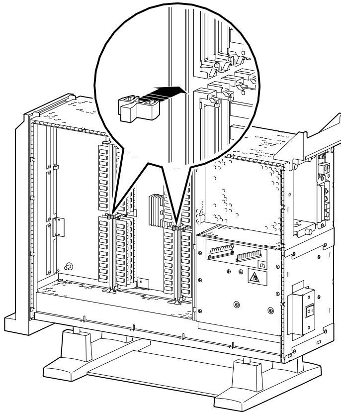
Figure 9–17 Installing MMB Clips
