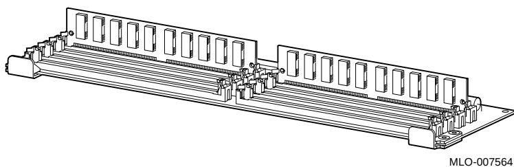
Figure 9–2 Memory Mother Board (MMB)
