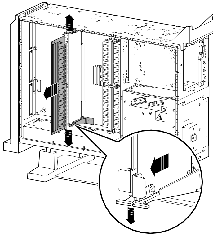
Figure 9–6 Removing an MMB
