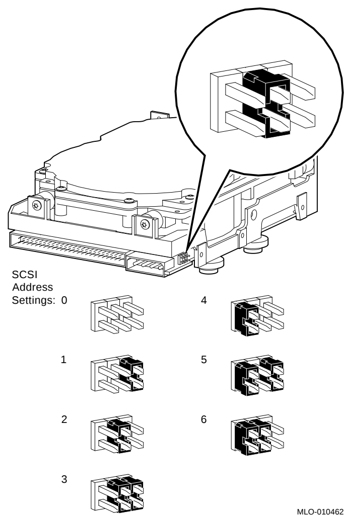
Figure 7-2 RZ25 SCSI Address Jumpers
