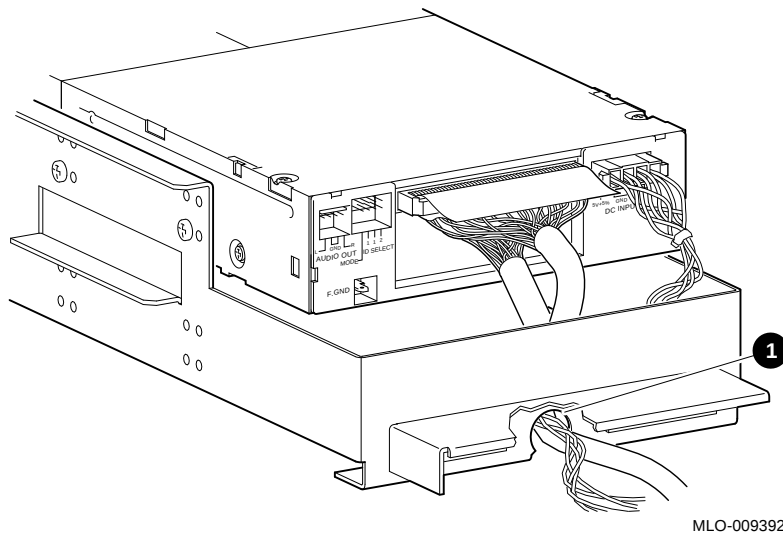
Figure 3-9 Slipping Cables into the Slot
