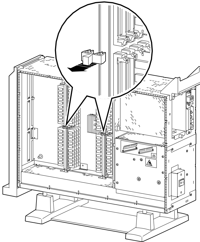
Figure 9–5 Removing MMB Clips
