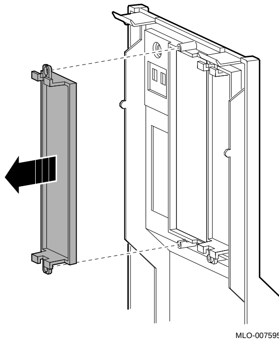
Figure 5–13 Removing the Blank Filler Plate from the Front Panel
