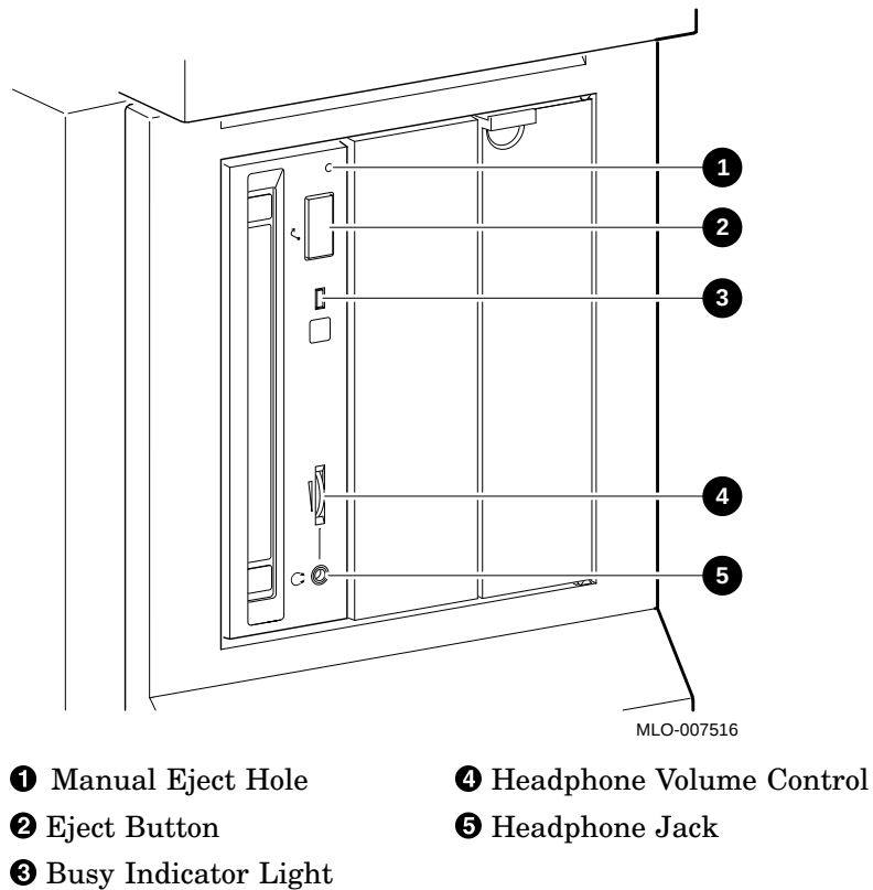
Figure 3–14 RRD42 Drive Controls and Indicators
