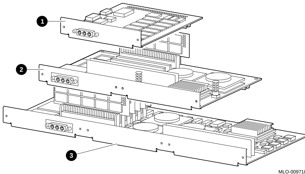
Figure 10–2 TURBOchannel Option Widths
