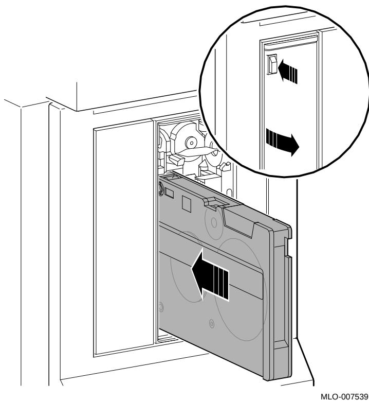
Figure 5-16 Inserting the TZK10 Tape Cartridge
