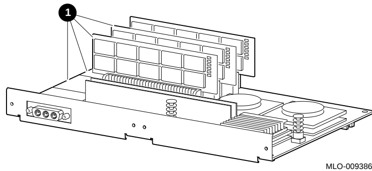
Figure 10-6 PXG+ 24-Plane 3D Graphics Module
