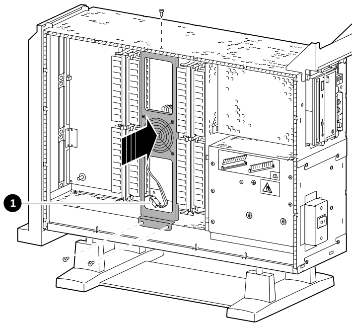
Figure 9–18 Installing the Fan Bracket
