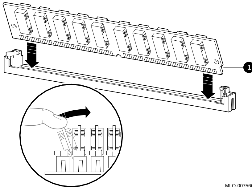
Figure 9–8 Installing a Memory Module
