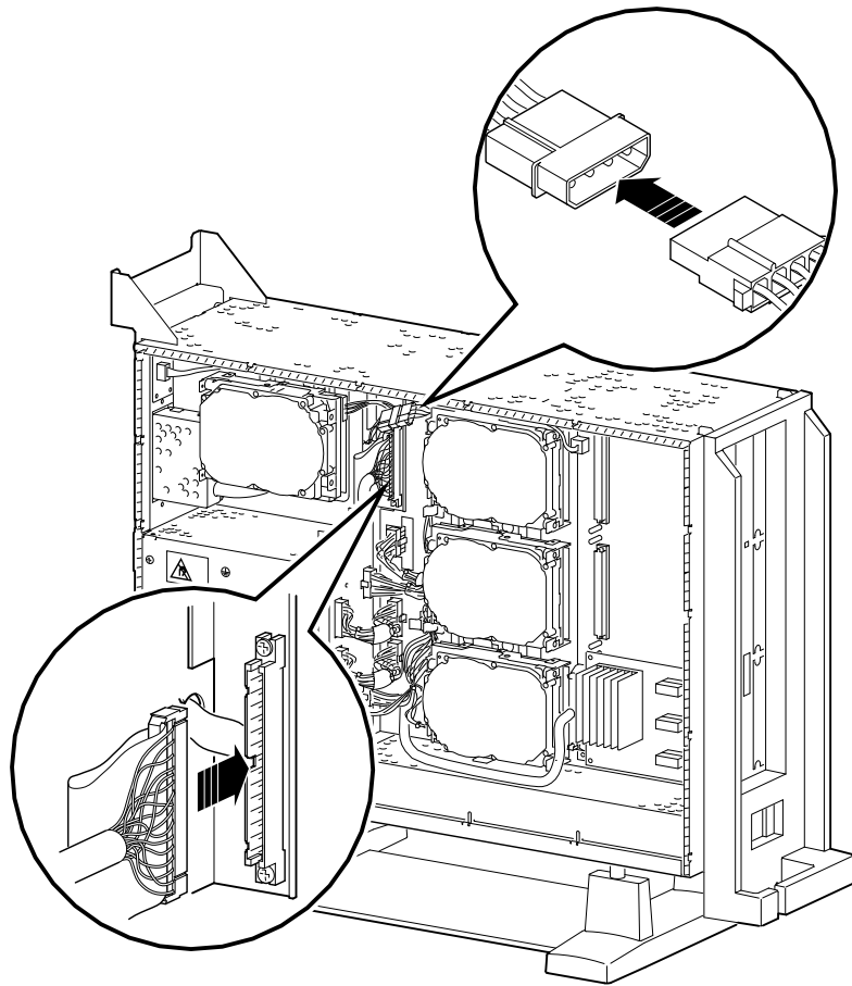
Figure 4–13 Connecting Cables
