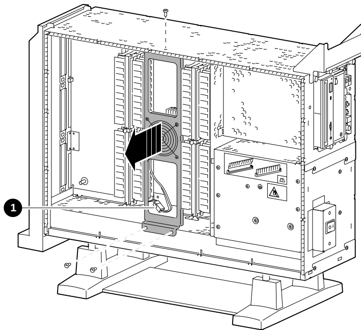
Figure 9–4 Removing the Fan Bracket
