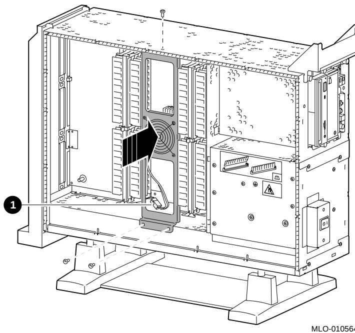
Figure 9-11 Installing the Fan Bracket
