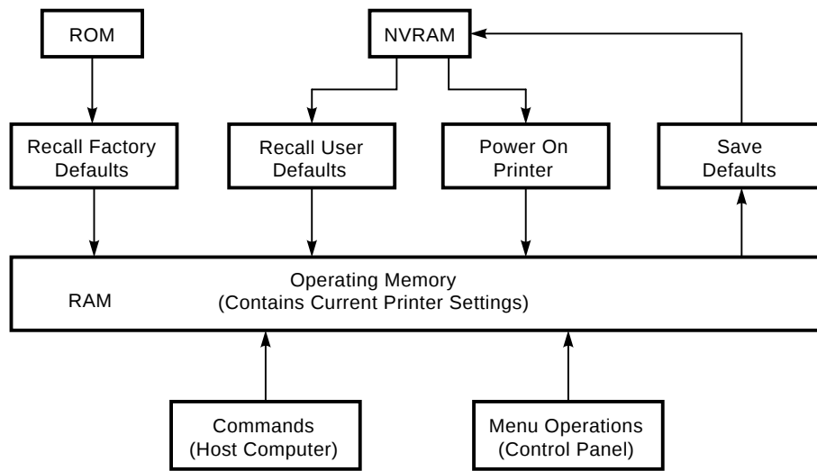
Figure 4-3 Operating Flow
