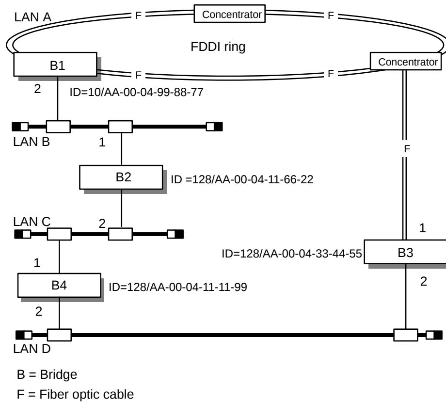
Figure 3–3: Determining the Root and Designated Bridges in a Looped Configuration
