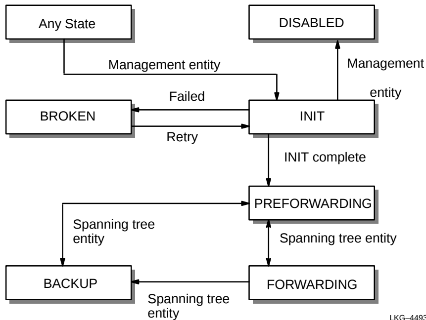
Figure 2–3: Port State Transitions
