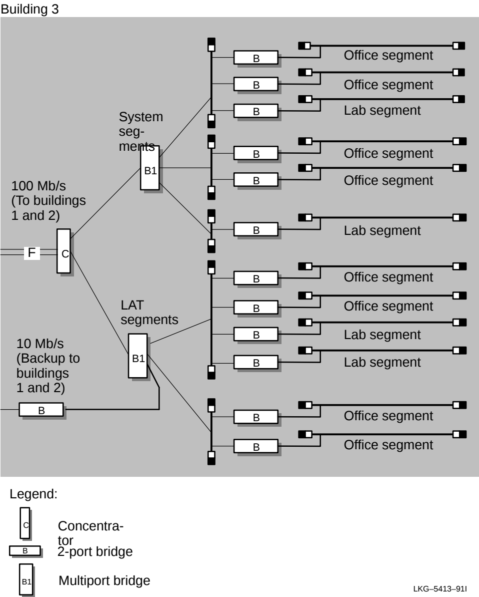
Figure 6-19: Extended LAN Example (Building 3)
