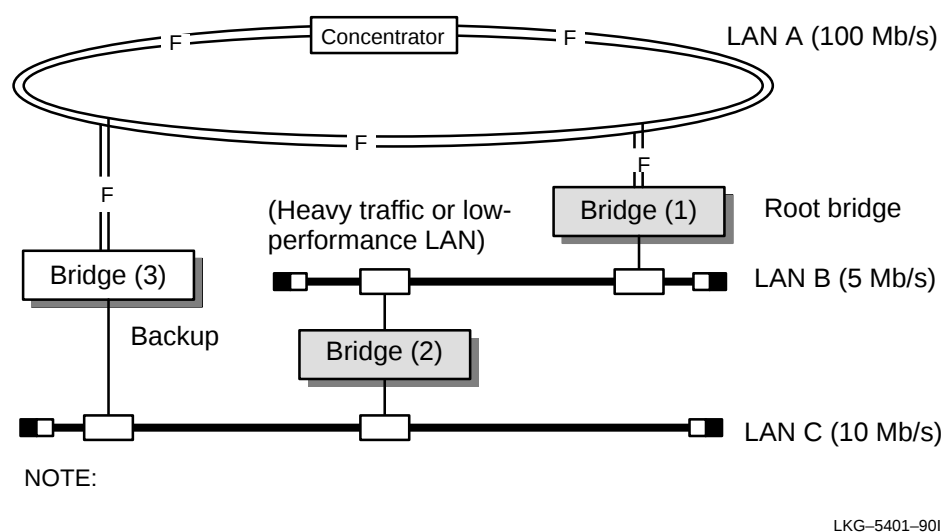
Figure 6–3: Example 1—Inefficient Bridge Configurations
