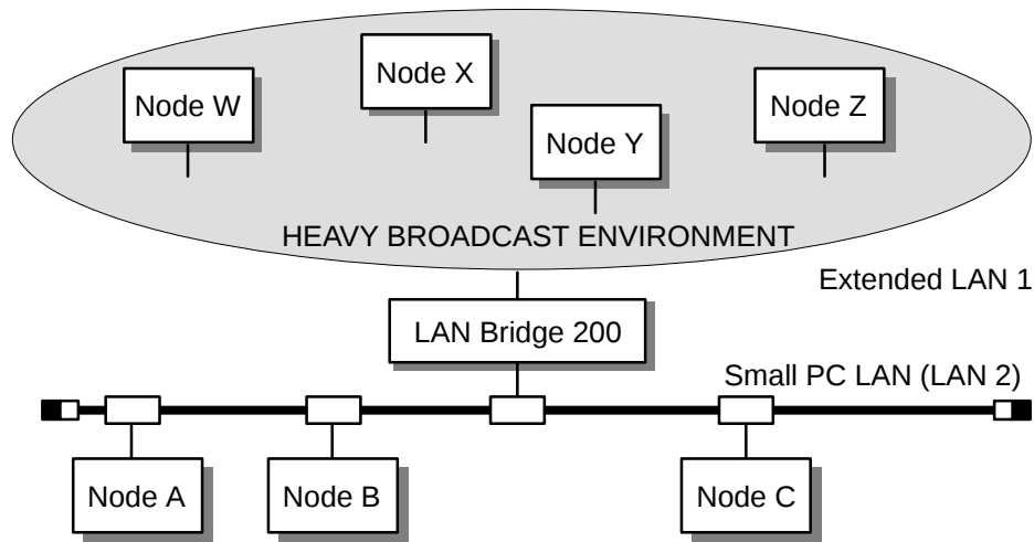
Figure 6-6: Example 1—Heavy Broadcast Traffic
