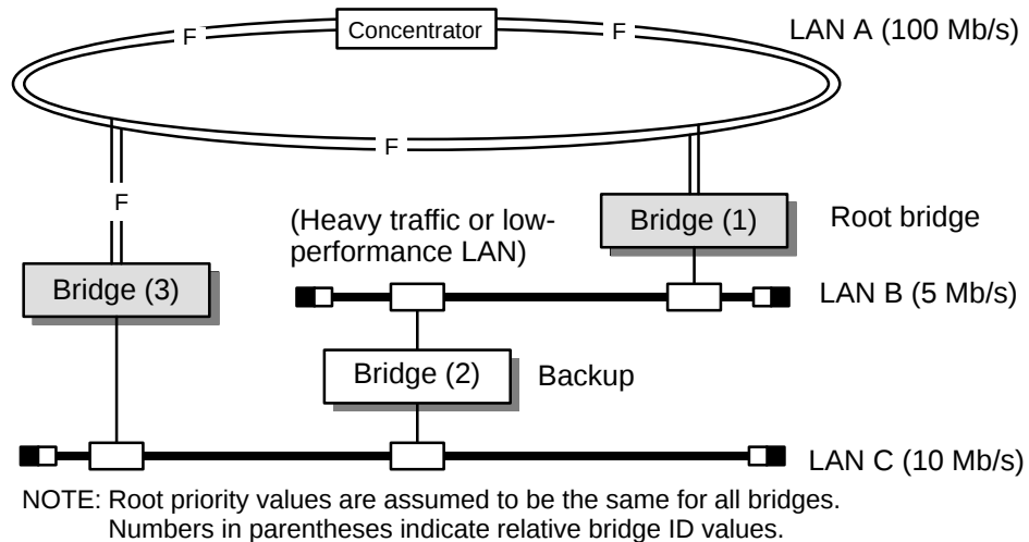
Figure 6-4: Example 1—A More Efficient Configuration
