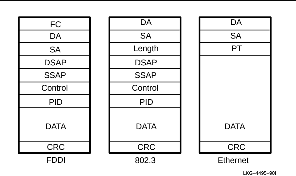
Figure 2–5: Frame Formats
