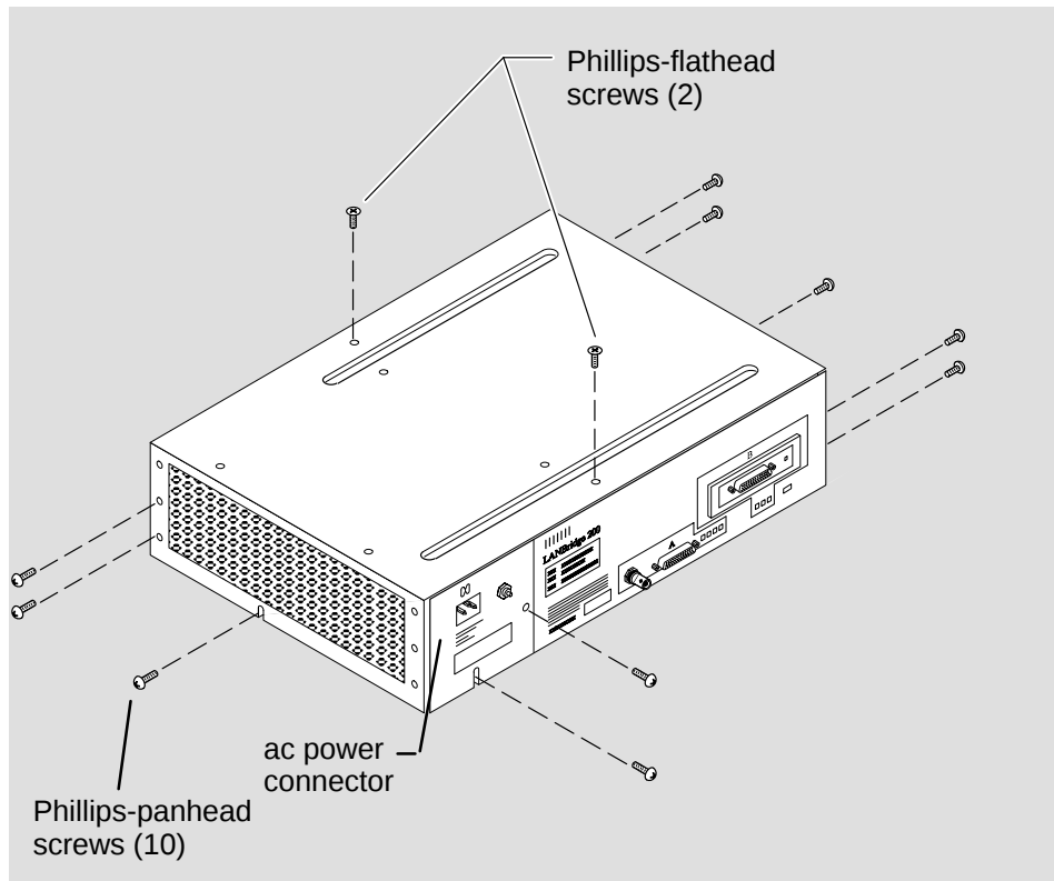
Figure 1–3: Removing Chassis Screws
