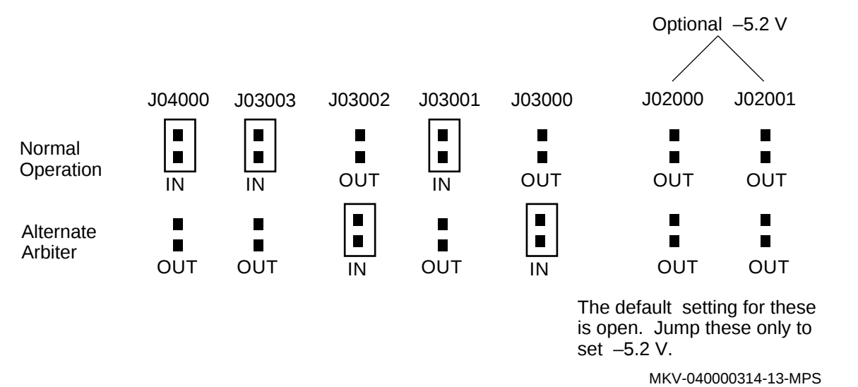
Figure 2–2 Parallel VME 6U Adapter Jumper Settings
