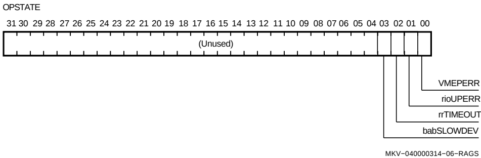
Figure 1–6 Parallel VME State CSR (OPSTATE)
