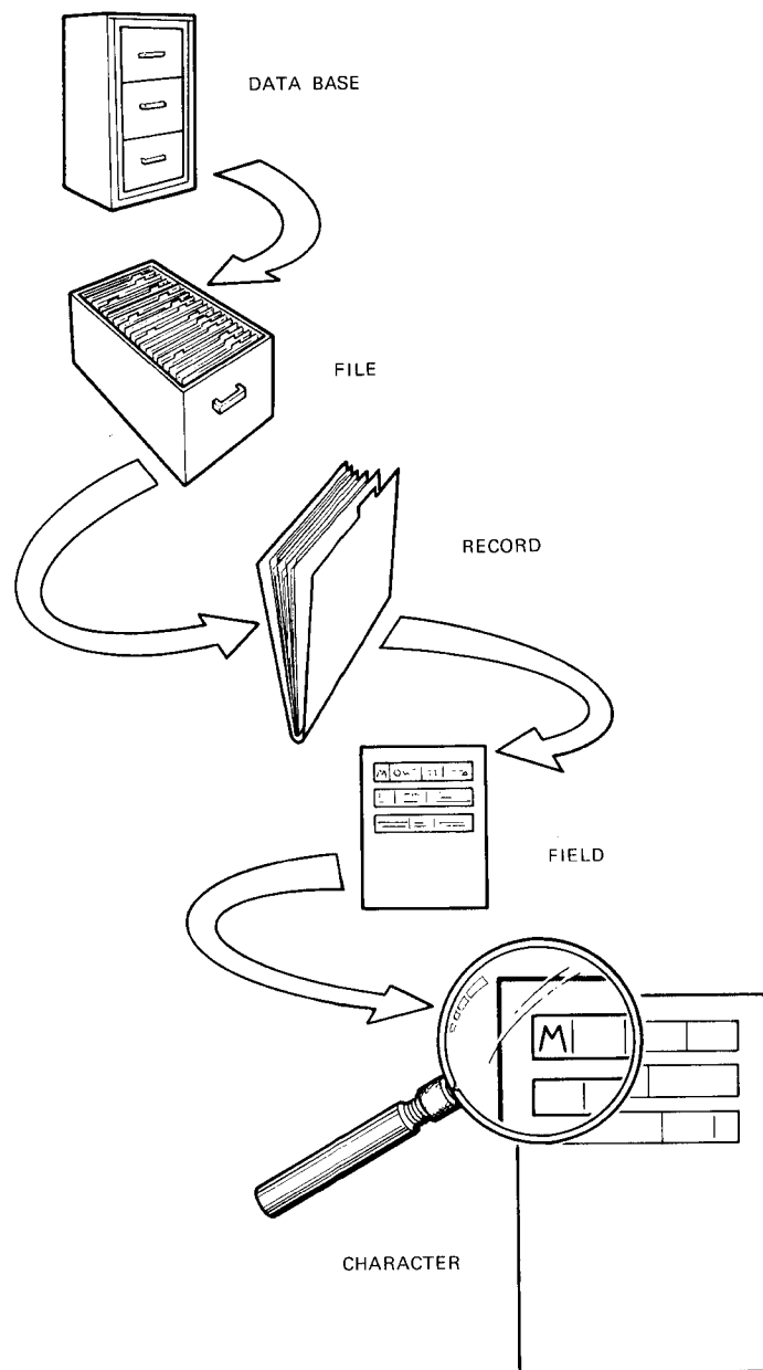
Figure 2-1 Data Hierarchy
