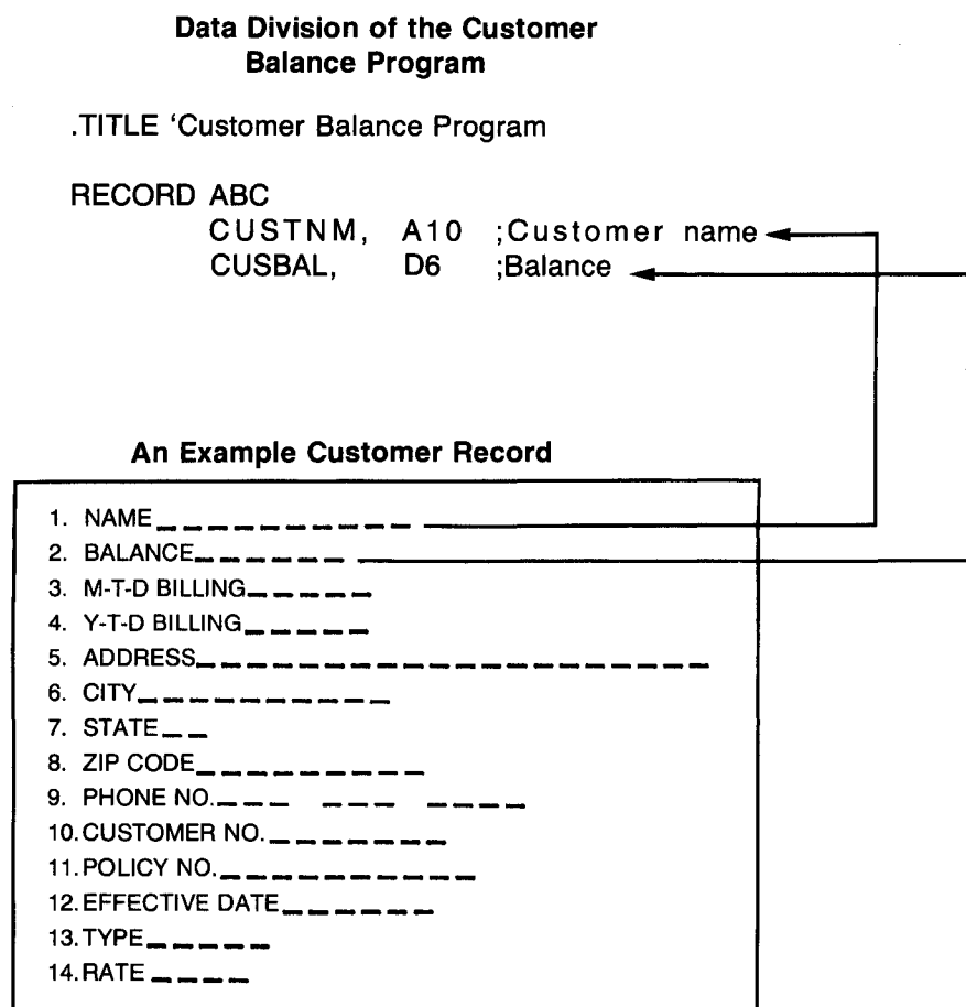
Figure 6-1 Customer Record/Data Division
