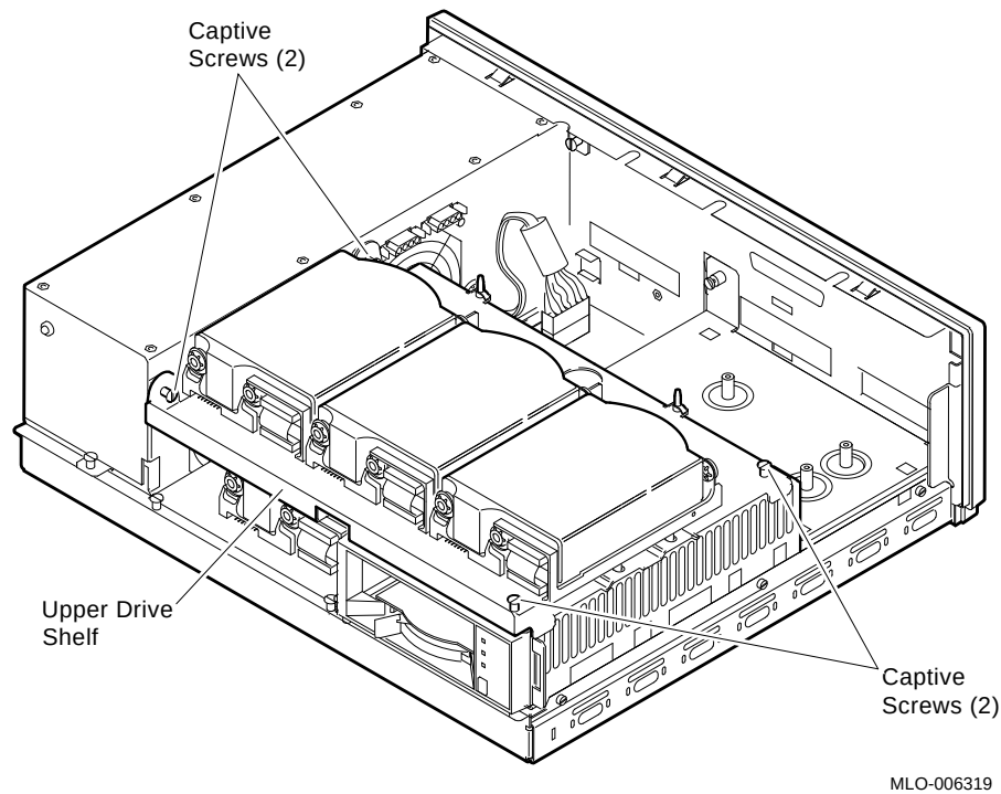
Figure 2-4: Removing Upper Drive Shelf
