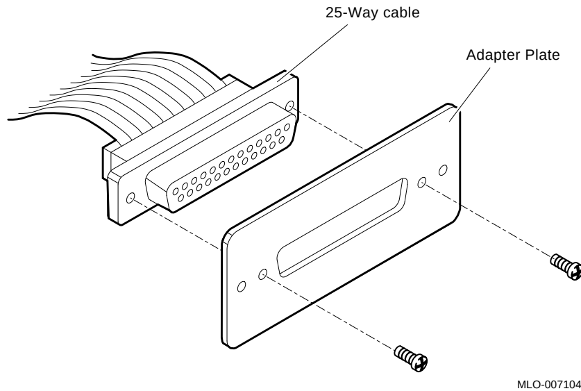
Figure 2-9: Attaching Modem Cable to Adapter Plate
