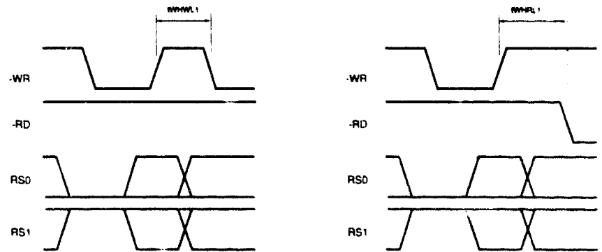
Figure 8-6. Microprocessor Interface Timing Model II
