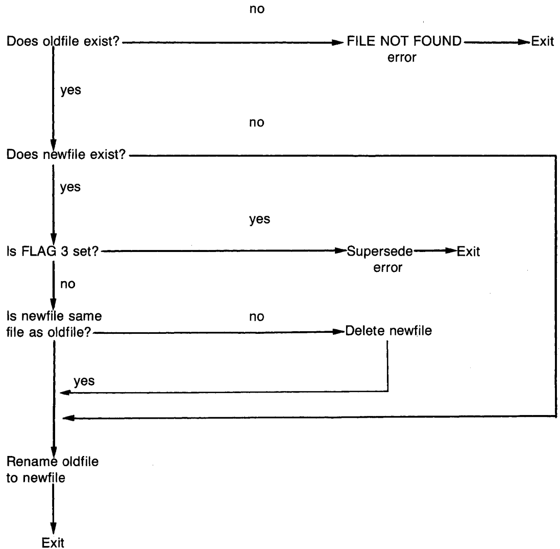
Figure 5-2 RENAM Flowchart
