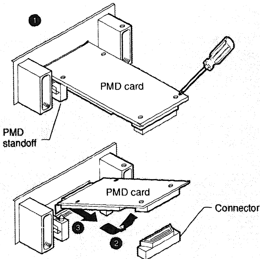
Figure B-1: Removing the PMD Card
