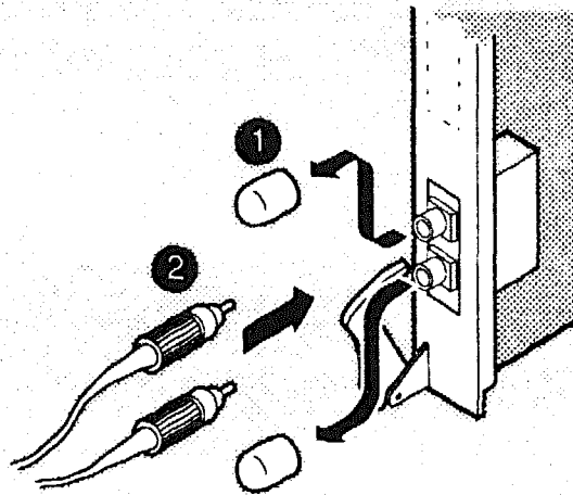
Figure 3-4: Connecting FDDI Single-Mode Cables
