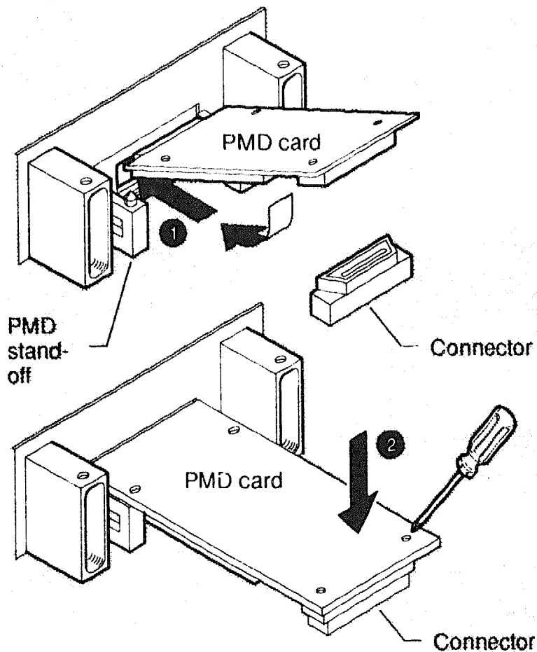
Figure B-3: Installing the PMD Card
