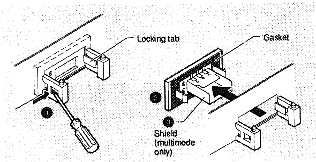
Figure B-2: Removing the Bezel
