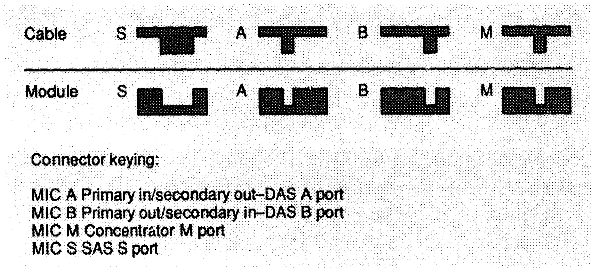
Figure C-1: Controller MIC Receptacle Keying
