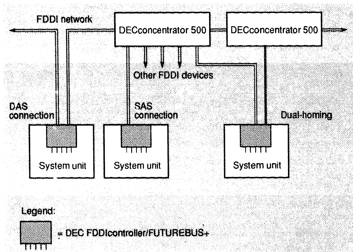
Figure 1-2: Connecting the DEC FDDIcontroller/FUTUREBUS+ to the FDDI Network
