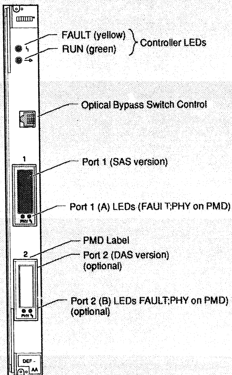
Figure 1-1: DEC FDDIcontroller/FUTUREBUS+
