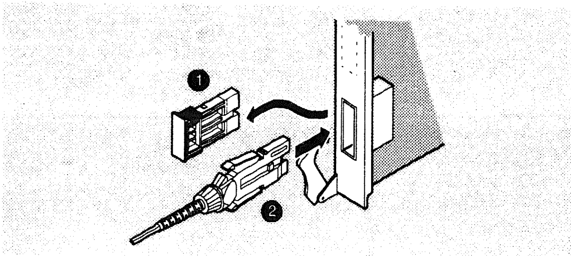
Figure 3-3: Connecting FDDI Multimode Cables
