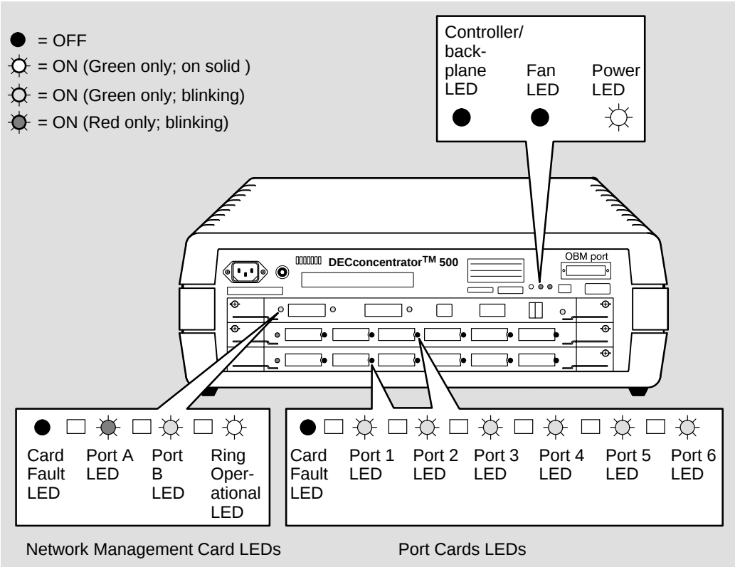
Figure 3-3: Port LED Status During Loopback Testing
