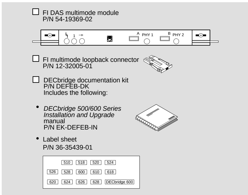
Figure 2–1: DEFEB-UP Upgrade Kit Contents
