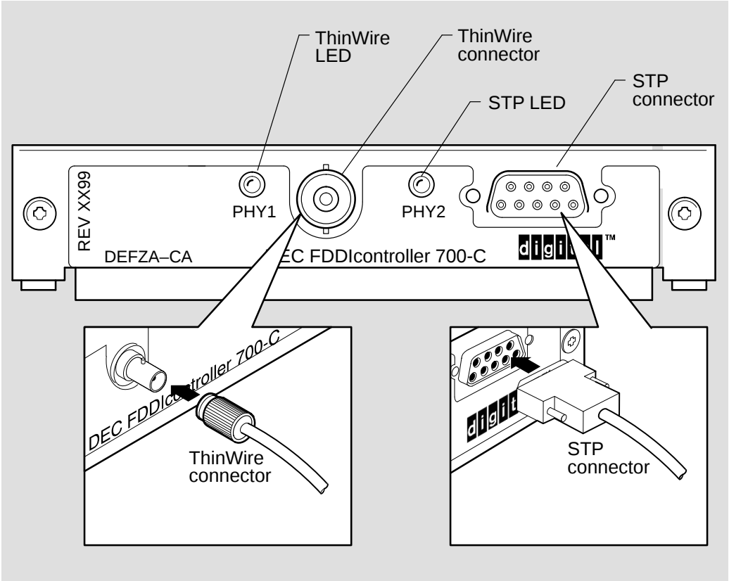
Figure 2-5: Example of Connecting the ThinWire and STP Connectors
