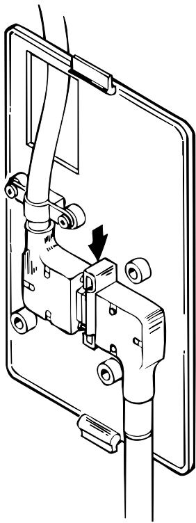
Figure A-5 Closing the Connector Latch
