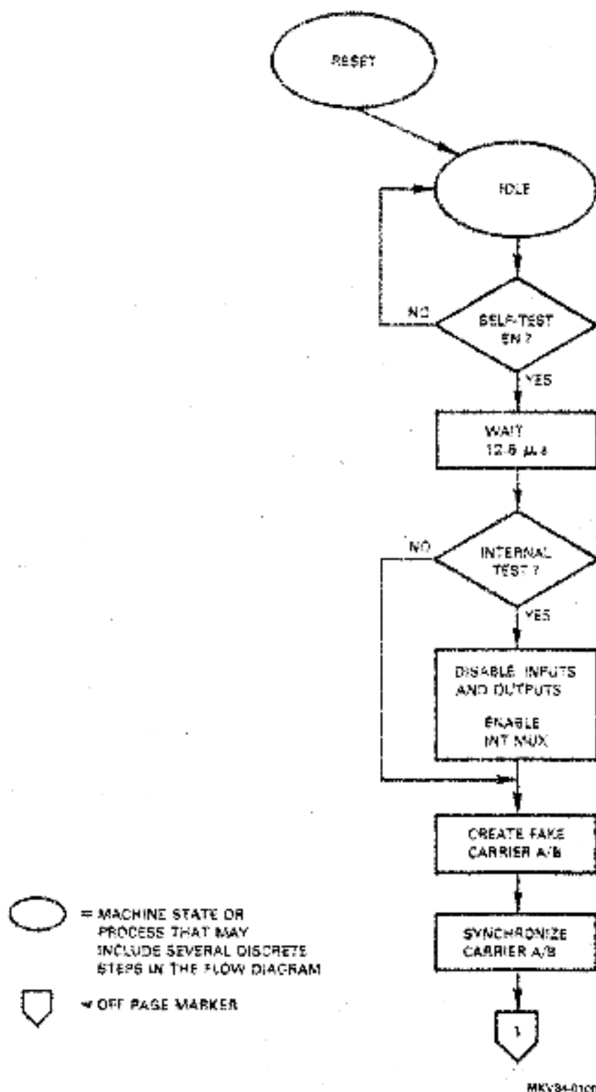
Figure 3-3 Internal Self-Test Flow Diagram (Sheet 1 of 5)
