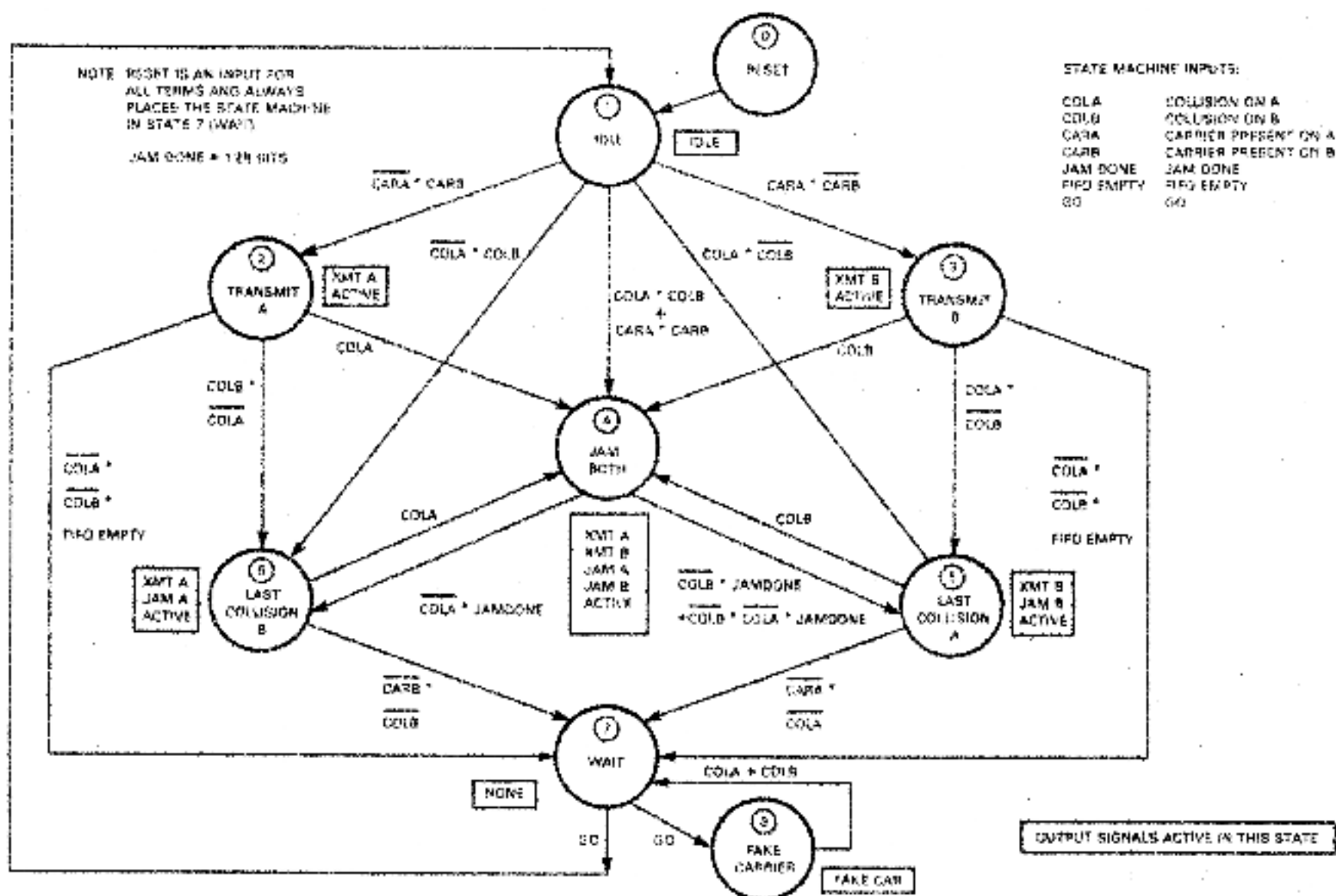
Figure 3-1 State Machine Flow Diagram
