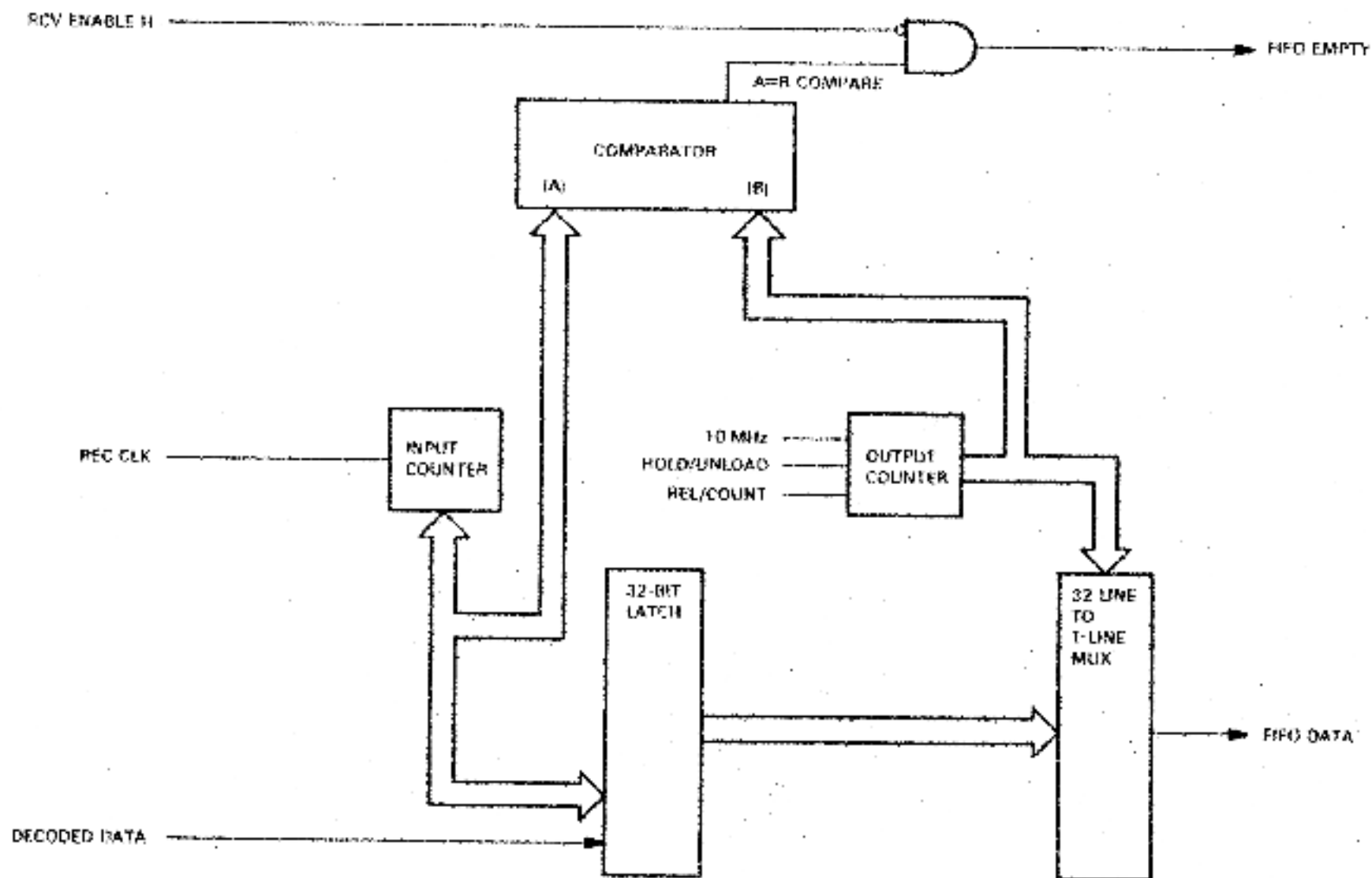
Figure 4-5 FIFO Block Diagram
