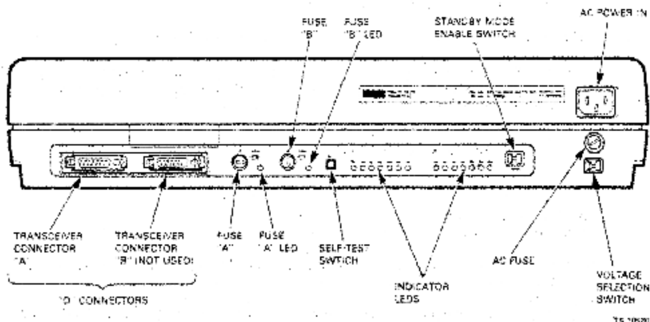
Figure 2-3 Local Repeater Rear Panel
