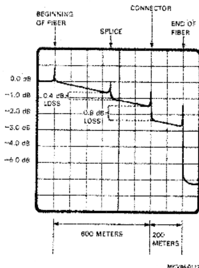
Figure A-2 Typical FOTDR Trace Showing a Splice and Connector
