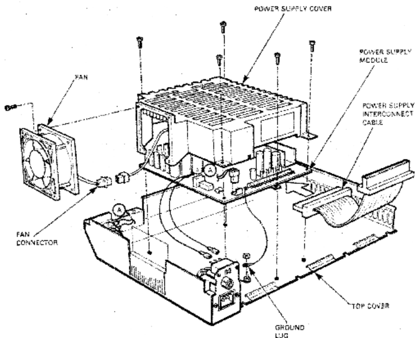
Figure S-10 Power Supply Chassis
