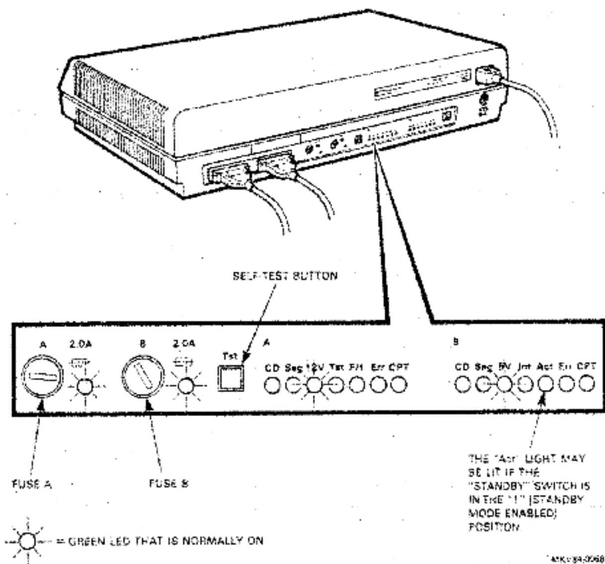
Figure S-3 Typical LED Status
