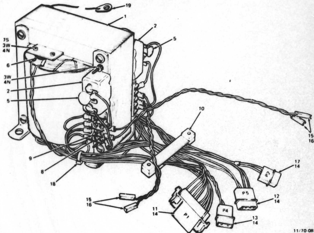
Figure 6. Transformer Assembly
