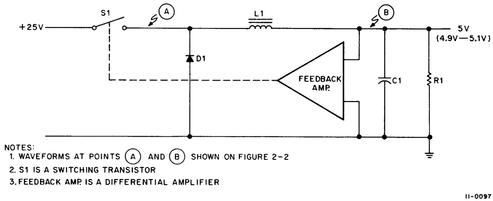
Figure 2-1 +5 Volt Regulator (Simplified Schematic)
