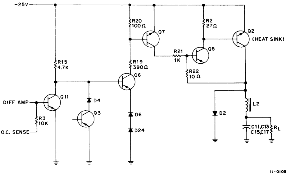
Figure 2-10 -15 Volt Driver
