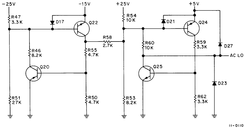
Figure 2-15 AC LO Circuit Schematic
