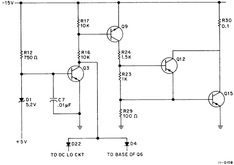
Figure 2-13 -15V Crowbar Circuit
