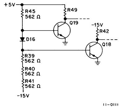
Figure 2-16 DC LO – Simplified Schematic
