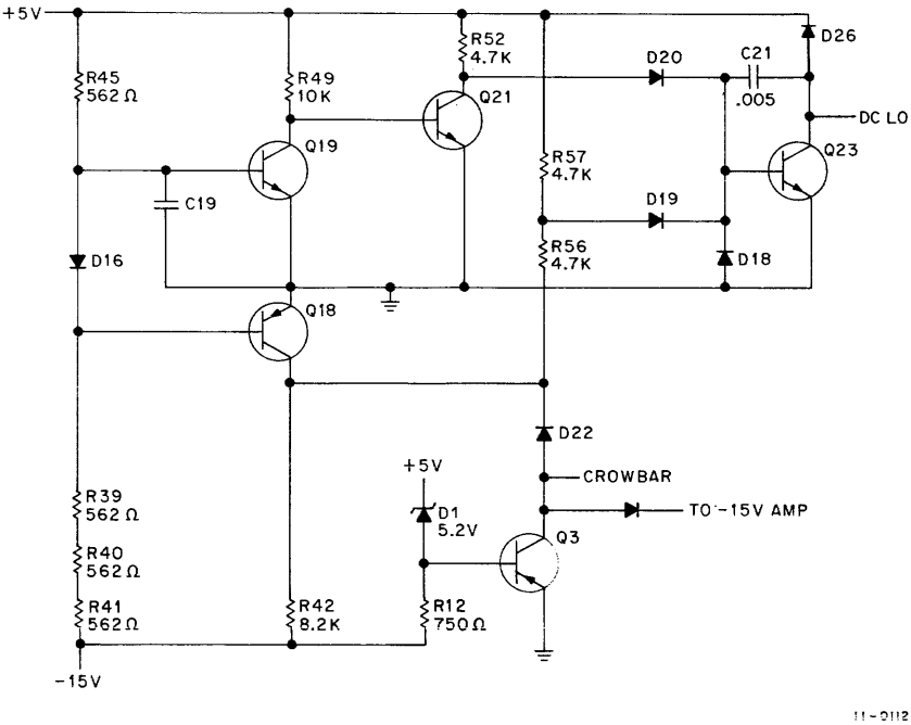
Figure 2-17 DC LO – Circuit Schematic
