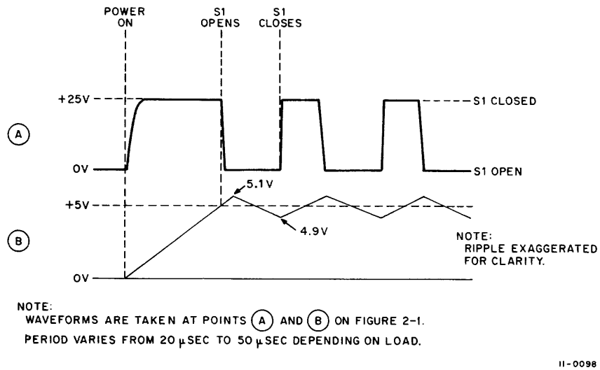
Figure 2-2 +5 Volt Regulator Waveforms
