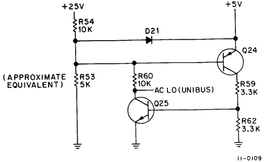
Figure 2-14 AC LO – Simplified Schematic
