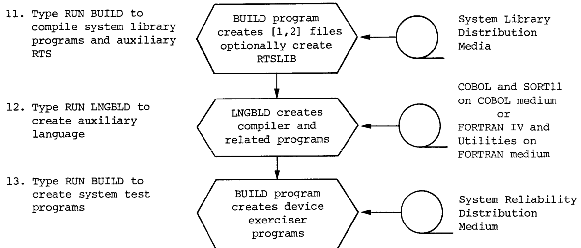
Figure 1-1 (Cont.) System Generation Flow Chart
