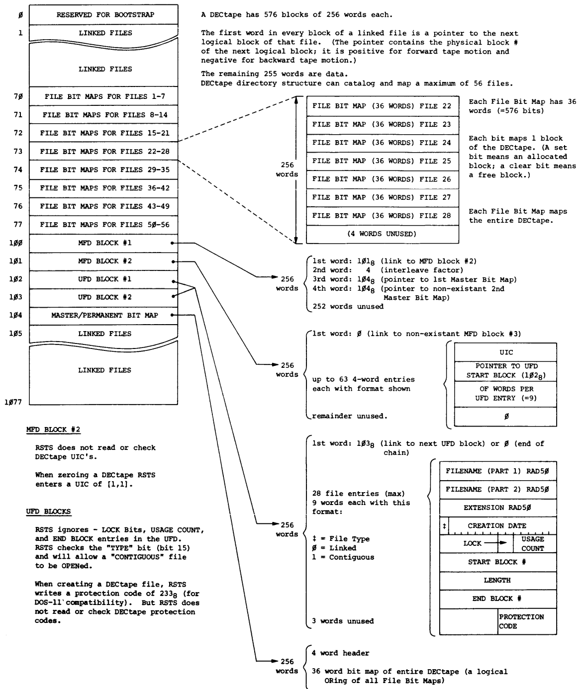
Figure 5-1 DECTape Format
