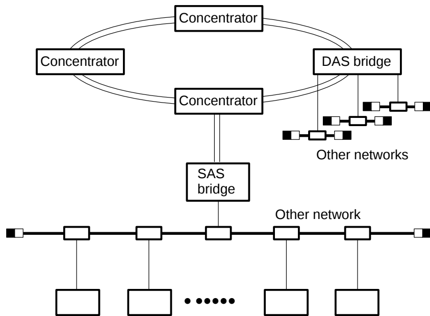
Figure 4–1: Extended LAN Examples
