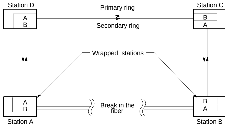
Figure 2–18: FDDI Typical Ring Recovery
