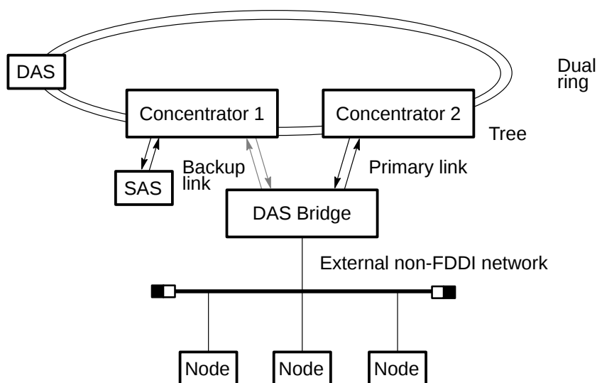
Figure 1–18: Dual Homing Topology Using Concentrators and a DAS Bridge
