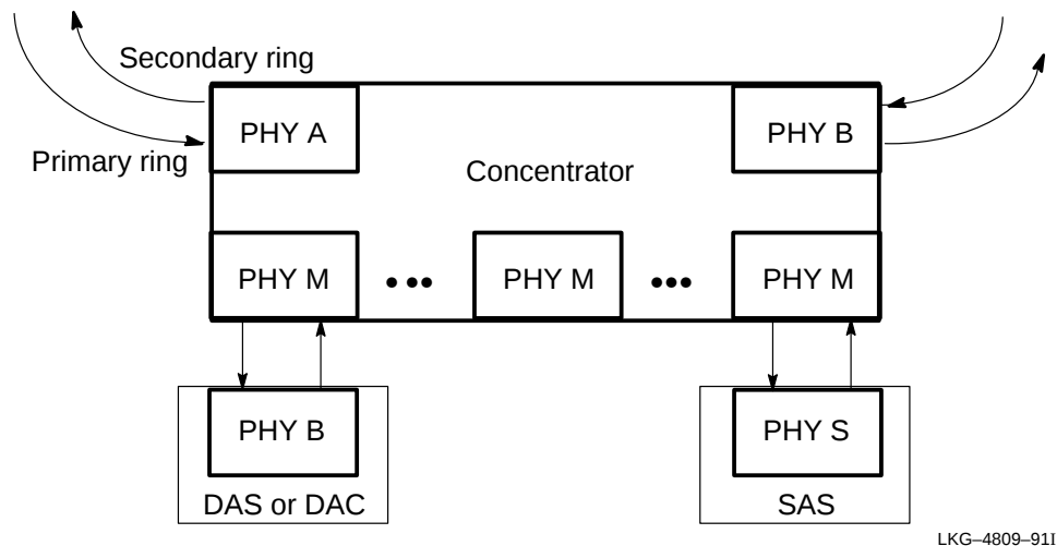
Figure 2–12: PHY- Port Types
