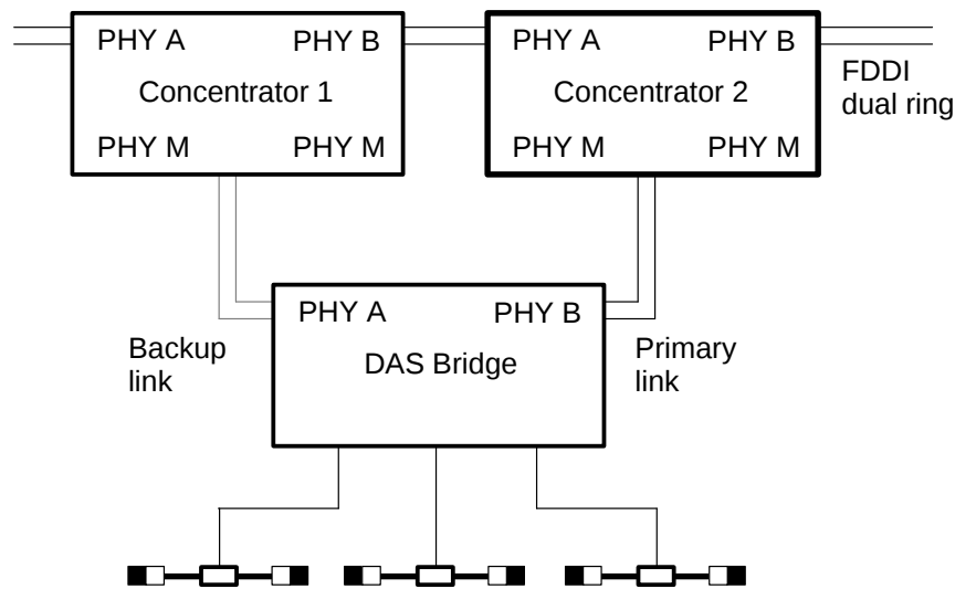
Figure B-8: DAS Bridge Installed for Dual Homing
