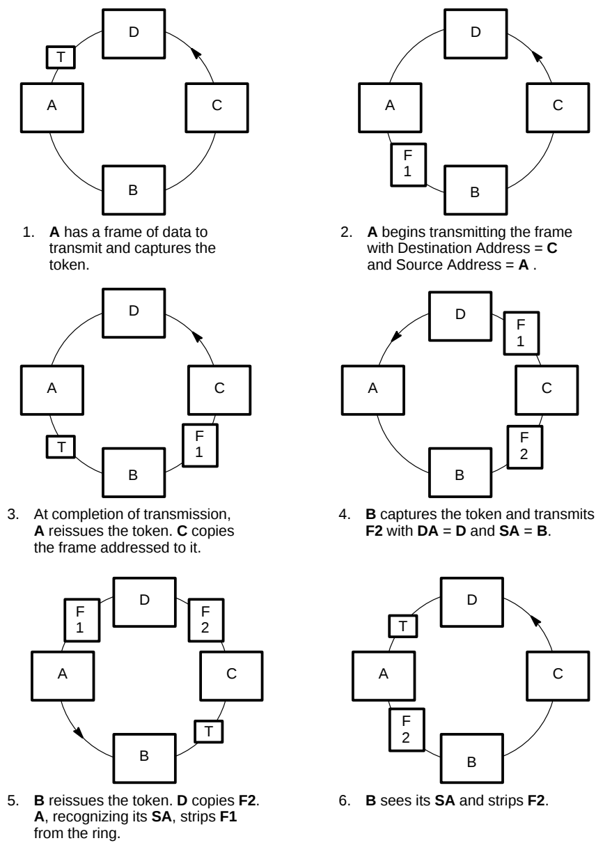
Figure 2-17: Capturing the Token
