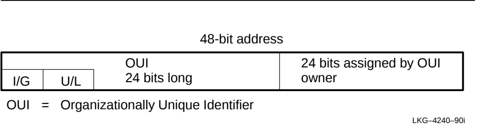
Figure 2-7: Universal Address Format
